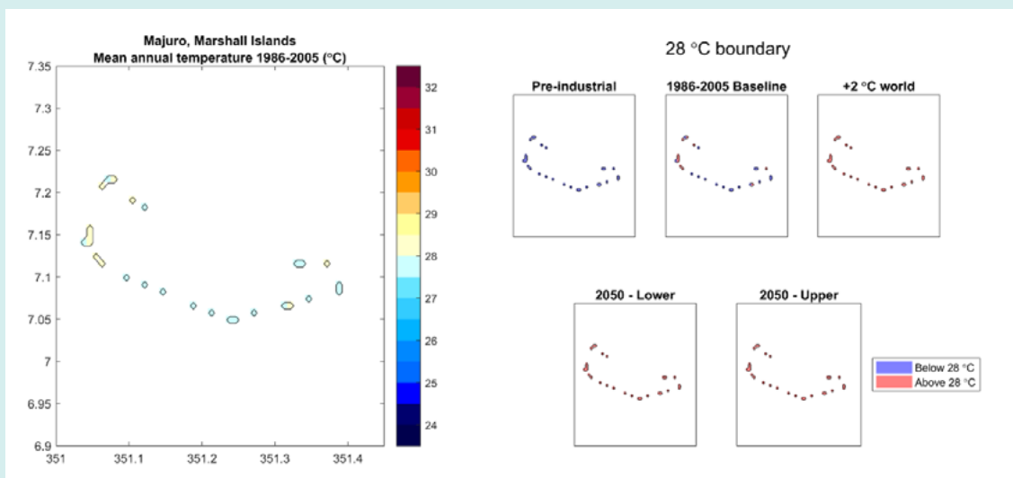
Figure 7.1. The average annual temperature in 1986-2005 in Majuro (left: the 'WorldClim' high-resolution climate surface adjusted for the baseline used), and the area of the island above or below the 28°C boundary for various scenarios (right).
