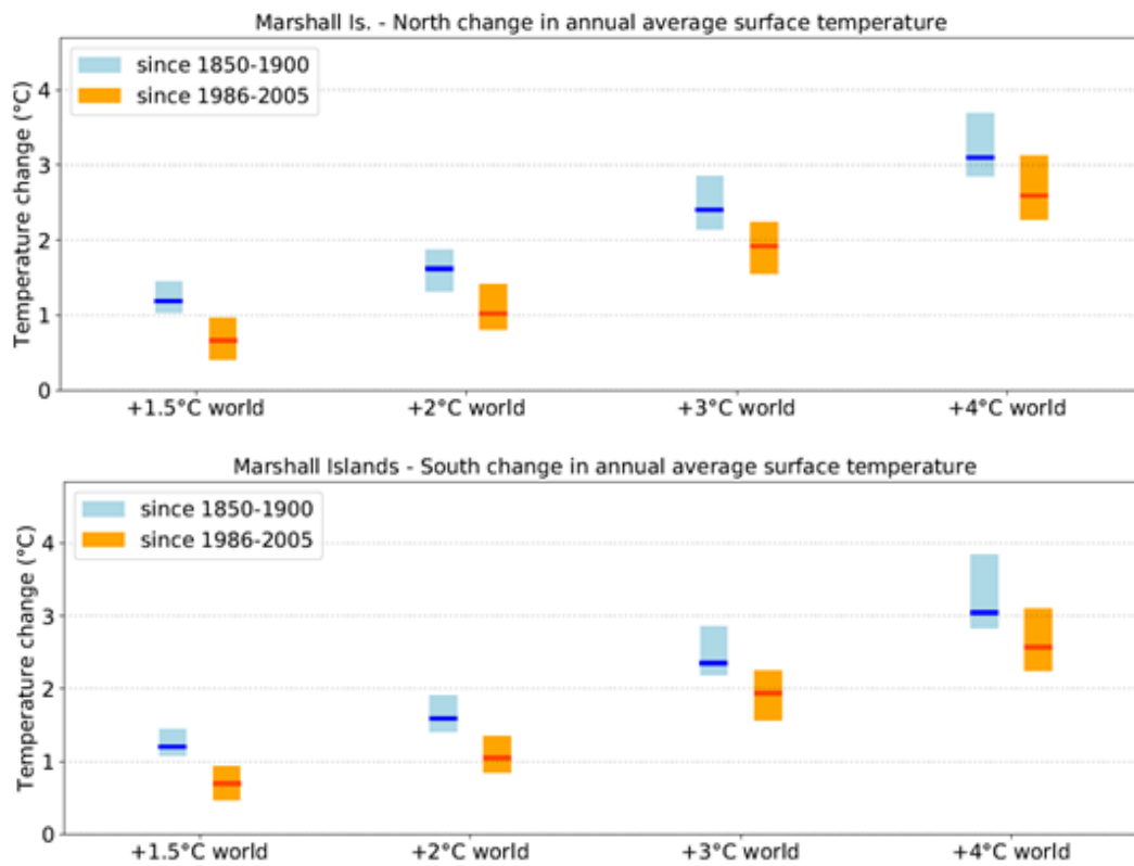
Figure 4.5. Change in the average annual temperature of Marshall Islands north and south regions at different global warming levels, from the 1850-1900 baseline, and from the more recent baseline of 1986-2005. The bars represent multi-model median and 10th-90th percentile range.
