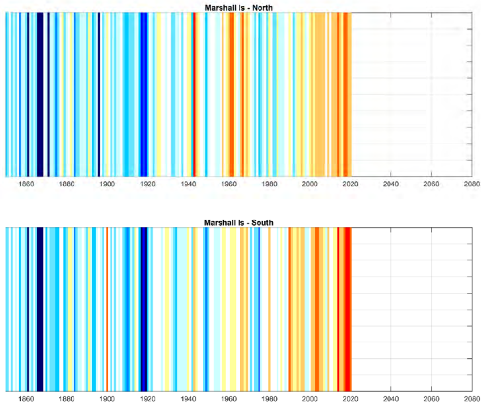
Figure 2.3 Marshall Islands north and south temperature relative to 1961-1990 through time presented as 'climate stripes' devised by Hawkins (2018): red = hotter, blue = cooler (using the Berkeley dataset).
