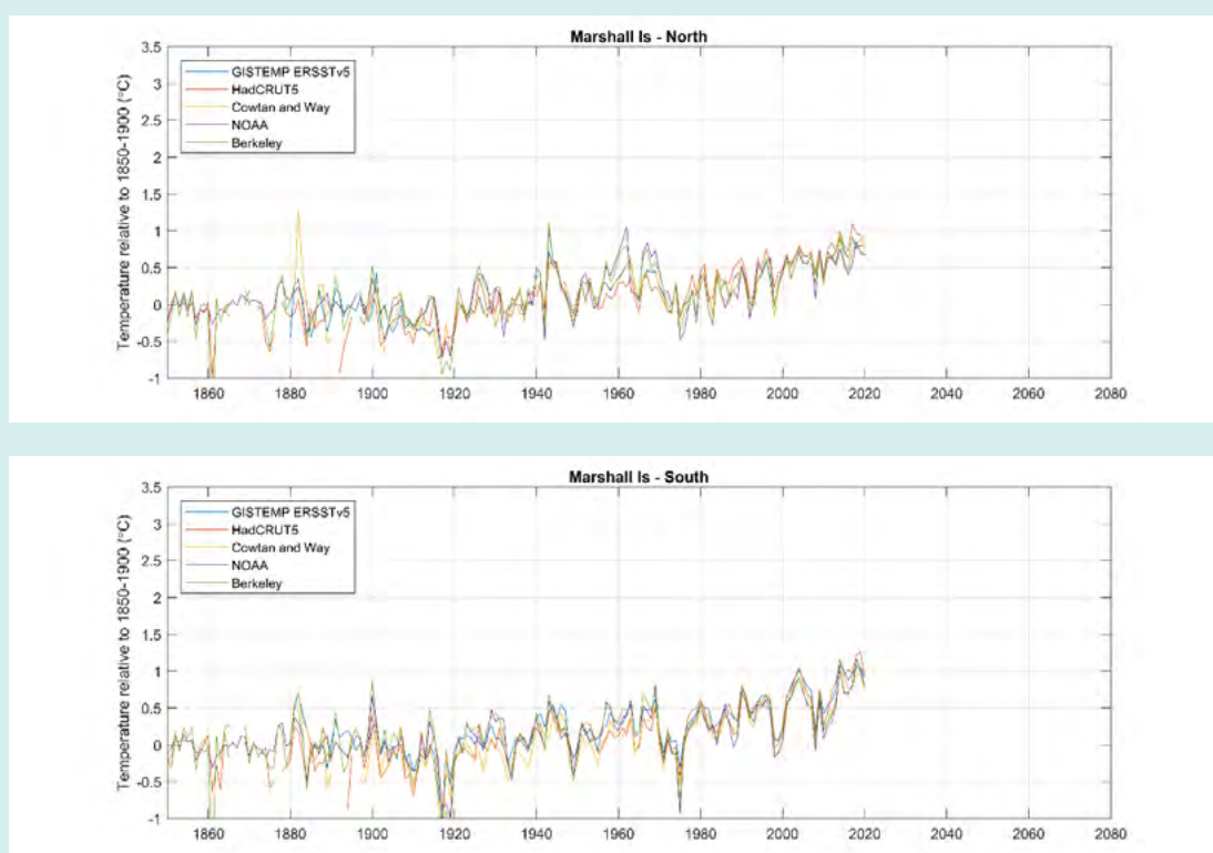
Figure 2.1. Average annual temperature of Marshall Islands north and south regions relative to 1850-1900 in five global datasets (see Methods, Section 8 for details).
