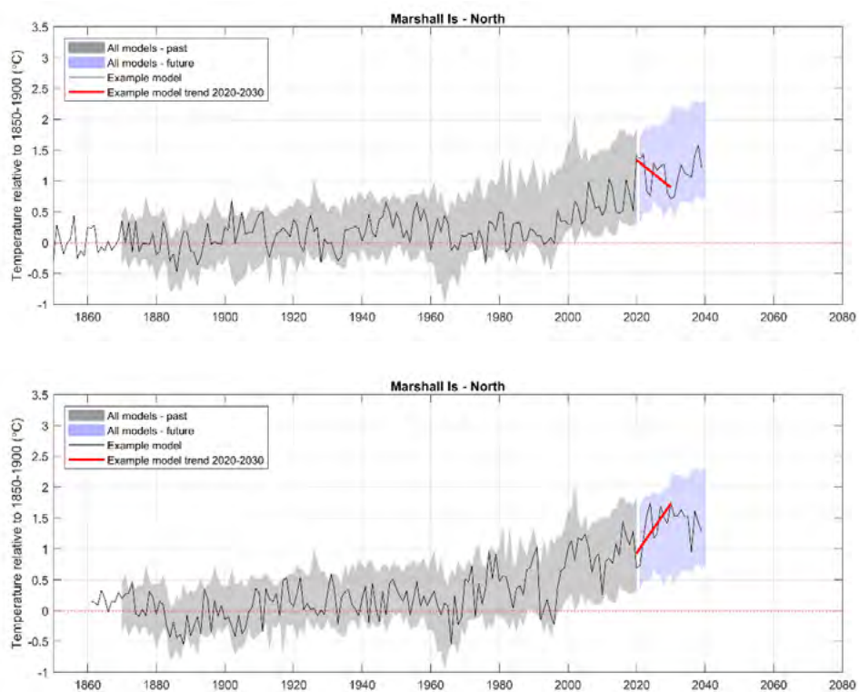
Figure 2.5. Average annual temperature in Marshall Islands North relative to 1850-1900 (°C) simulated in CMIP5 models, showing the range of all models (historic; grey band, future; blue band) and example model simulations (black line) with the linear trend for 2020-2030 marked (red line); top: an example with suppressed warming in 2020-2030 due to climate variability, bottom: an example where variability enhances the warming trend.
