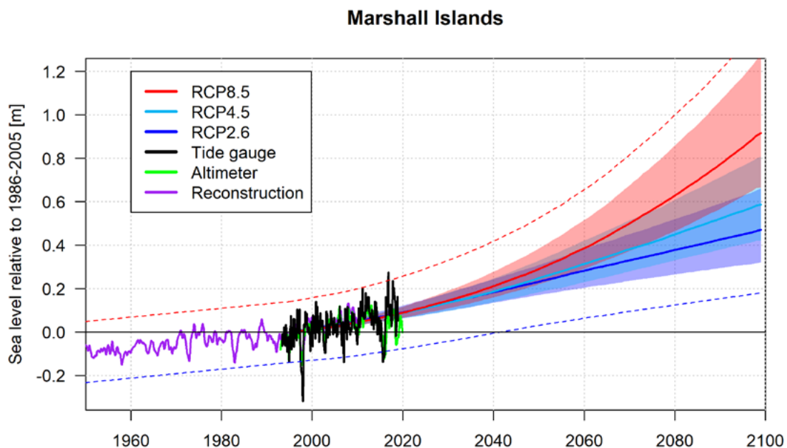
Figure 5.2 Sea level rise projections for Marshall Islands. The tide gauge record of relative sea level at Majuro is indicated in black, the satellite record in green and reconstructed sea level data is shown in purple, all are monthly means without seasonal cycles and referenced to mean sea level between 1986-2005. Multi-model-mean projections from 1995–2100 are given for the RCP8.5 (red solid line), RCP4.5 (cyan solid line) and RCP2.6 emissions scenarios (blue solid line), with the 5–95% uncertainty range for RCP8.5 and RCP2.6 shown by the red and blue shaded regions respectively. The dashed lines are an estimate of interannual variability in sea level (5–95% uncertainty range) and indicate that individual monthly averages of sea level can be above or below longer-term averages.
