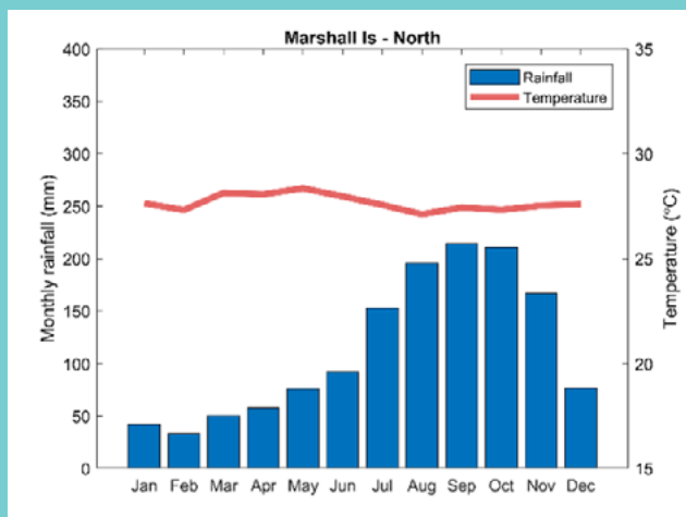
Figure 1.2. Mean annual cycle of rainfall and temperature in Marshall Islands north and south in 1981-2010 (rainfall uses ERA5, temperature uses HadCRUT5, see Methods in Section 8).
