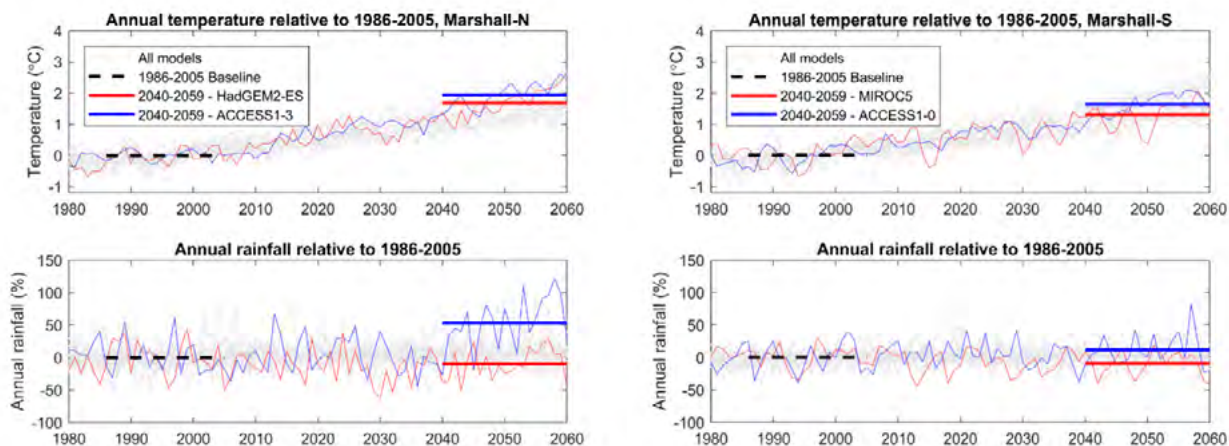
Figure 6.2 Modelled annual temperature (°C) and rainfall (%) changes in Marshall Islands north and south relative to 1986-2005 from CMIP5 models, showing the selected models that are representative of a warm dry future (red) and a hot wet future (blue).
