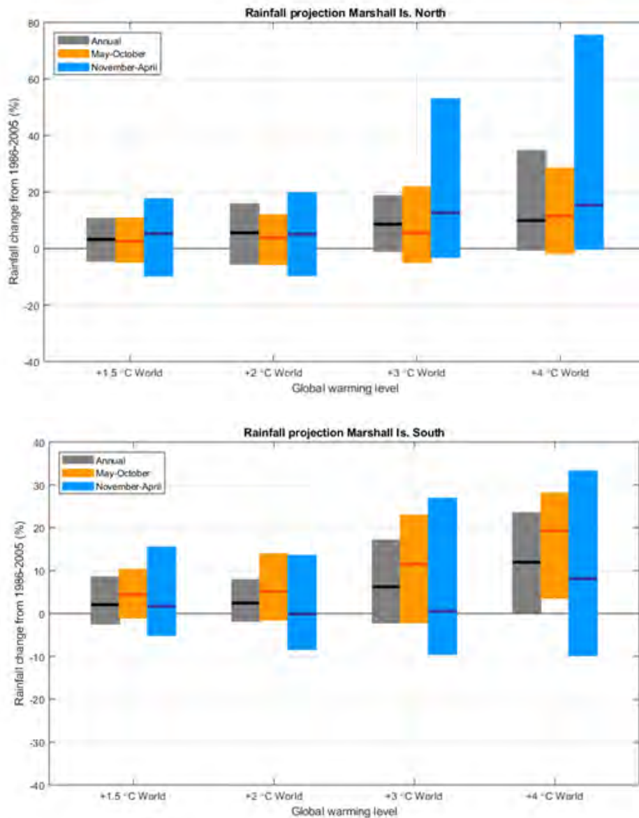
Figure 4.6. Change in the average annual and 6-month seasonal rainfall in Marshall Islands region at different global warming levels relative to the 1986-2005 baseline. The bars represent multi-model median and 10th-90th percentile range. Note expanded scale for Marshall Islands north to show the high end for higher warming levels.
