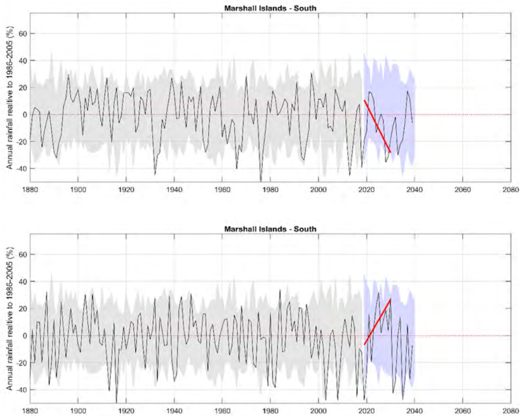
Figure 3.2 Mean annual rainfall of Marshall Islands south region relative to 1986-2005 (%) from the group of CMIP5 models (grey band: historic, blue band: future), with an example model run shown in each panel (black line) highlighting the different possible trend in 2021-2030: (top) a model showing a decrease (red trend line in the top panel), and (bottom) a model showing an increase (red trend line in the bottom panel).
