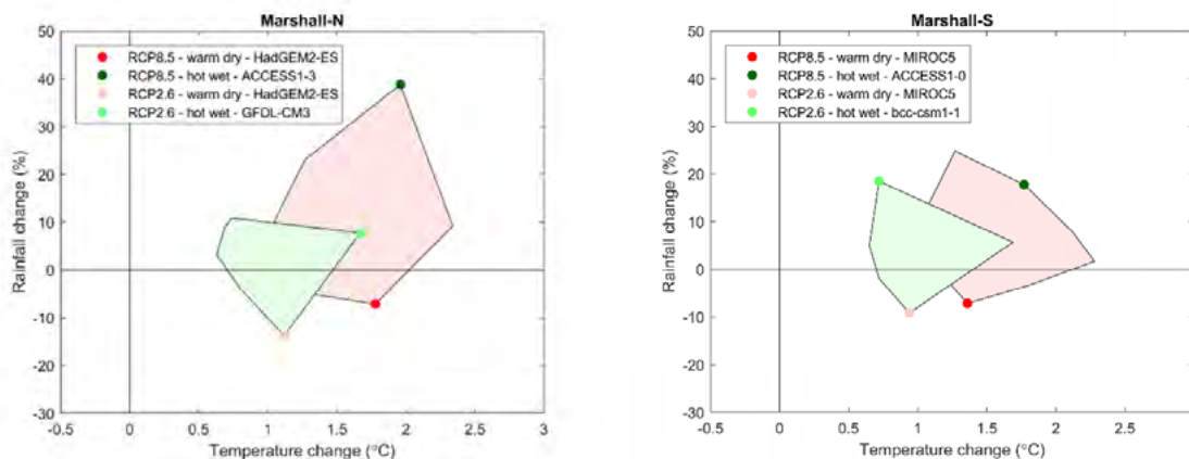
Figure 6.1 Modelled change in annual temperature and rainfall in Marshall Islands region between 1986-2005 and 2040-2059 from CMIP5 models (coloured shapes), showing the selected models that are representative of a warm dry future and a hot wet future for RCP2.6 (low case: green polygon) and RCP8.5 (high case: red polygon).
