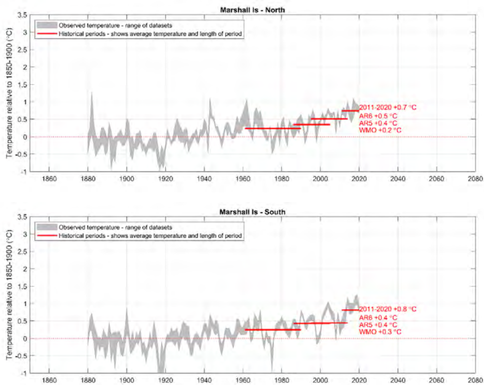
Figure 2.2 Average annual temperature of Marshall Islands north and south relative to 1850-1900 (°C; grey band indicates the range of five global temperature datasets) and the climate average for four different historical periods (baselines), as marked:
