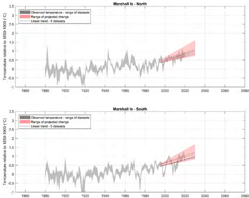
Figure 2.4 Average annual temperature of Marshall Islands north and south regions relative to 1850-1900 (°C; grey band indicates range of five global temperature datasets), the reported range of projected change from PACCSAP is shown as a red wedge (the starting point allows for the difference between the five datasets) and the linear trend of smoothed observations for 1995-2020 plotted and extrapolated forward to 2030 (one dotted line for each dataset).
