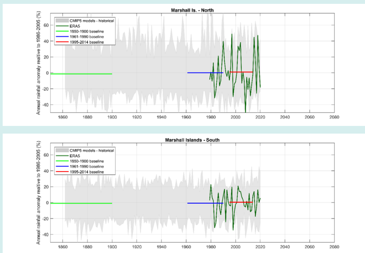
Figure 3.1 Area-average of Marshall Islands north and south annual rainfall (%) relative to the 1986-2005 period from gridded observations (ERA5 shown, results are similar from GPCP, CMAP and ERA5), the range of CMIP5 models (grey band). Coloured horizontal bars show the average of all models for the baseline periods described in the legend.
