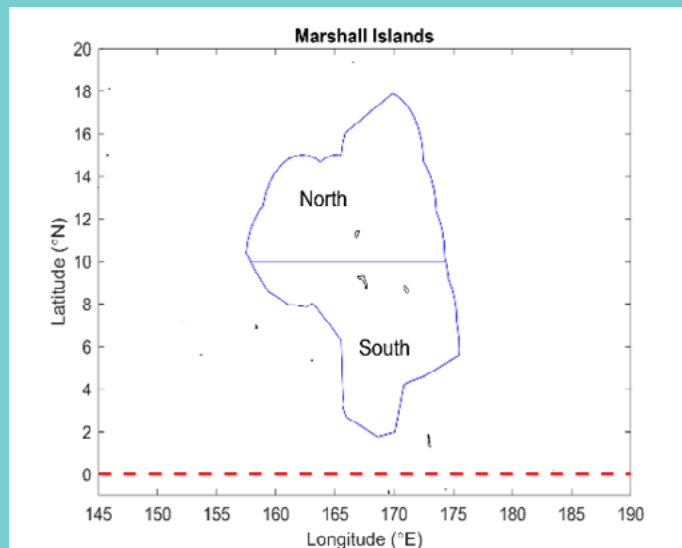
Figure 1.1. Map of Marshall Islands (top) and the mask area (centre) for calculating areal averages from gridded observational data and climate models' outputs.
