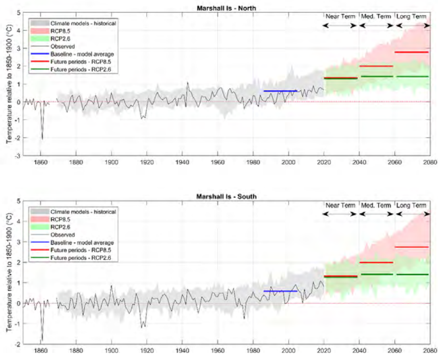
Figure 2.6. Average annual temperature in Marshall Islands north and south relative to 1850-1900 (°C) derived from observations (Berkeley shown; grey solid line) and simulated in CMIP5 models, showing the range of all models for the past period (grey band), the future under a very high emissions pathway (pink band) and a very low emissions pathway (green band). Thick horizontal lines show the mean of all models in 20-year periods of the baseline 1986-2005 (blue) and future 20-year periods centred on 2030, 2050 and 2070 (RCP8.5; red horizontal lines, RCP2.6; green horizontal lines).
