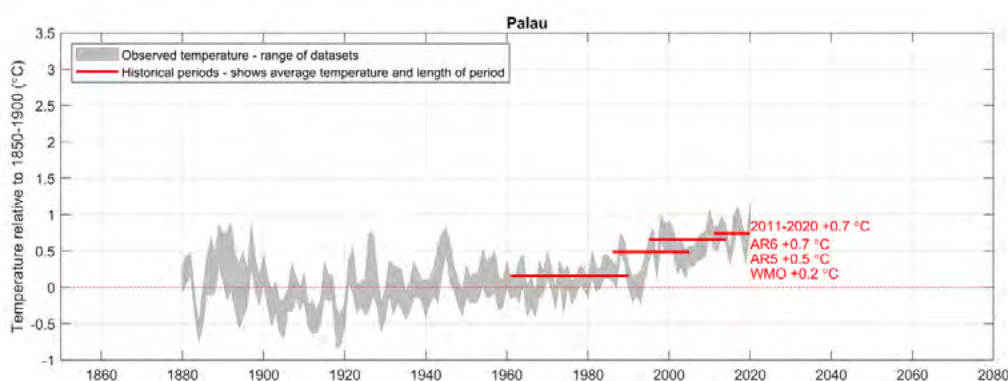
Figure 2.2 Average annual temperature of Palau relative to 1850-1900 (°C; grey band indicates the range of five global temperature datasets) and the climate average for four different historical periods (baselines), as marked:
