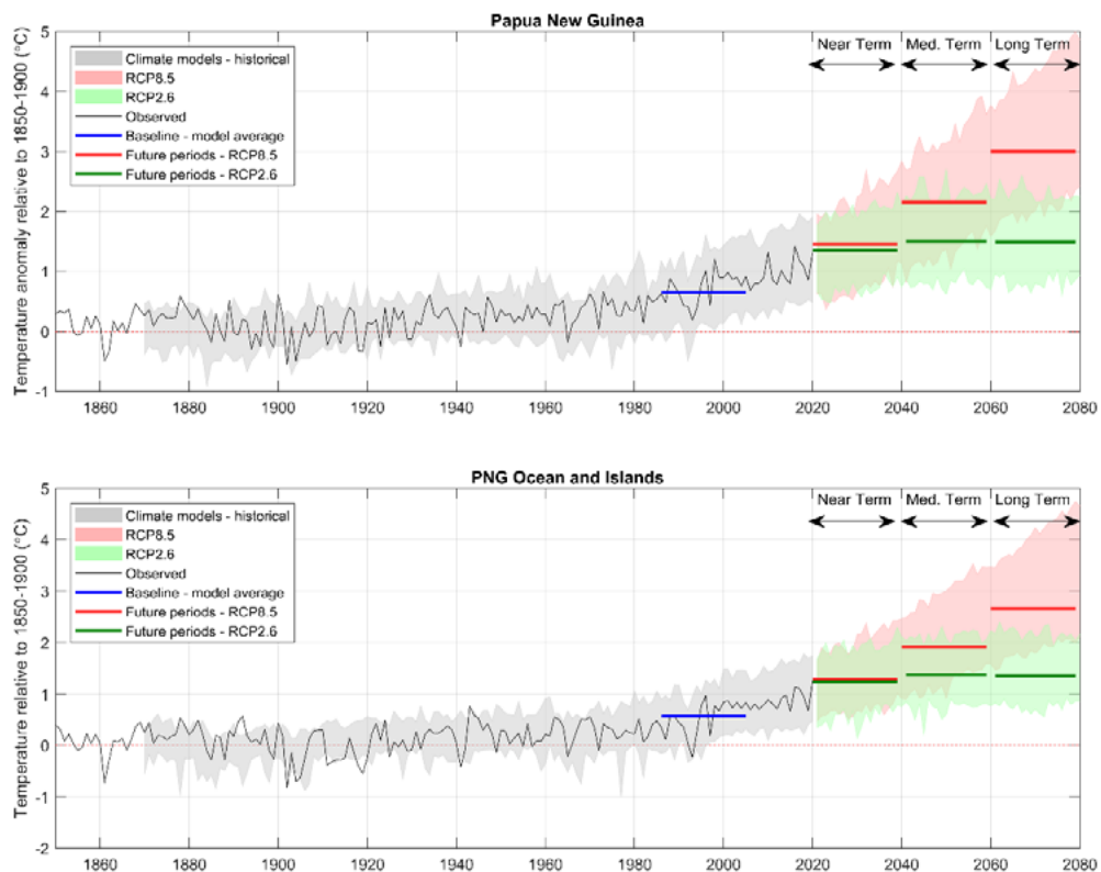
Figure 2.6. Average annual temperature in Papua New Guinea relative to 1850-1900 (°C) derived from observations (Berkeley shown; grey solid line) and simulated in CMIP5 models, showing the range of all models for the past period (grey band), the future under a very high emissions pathway (pink band) and a very low emissions pathway (green band). Thick horizontal lines show the mean of all models in 20-year periods of the baseline 1986-2005 (blue) and future 20-year periods centred on 2030, 2050 and 2070 (RCP8.5; red horizontal lines, RCP2.6; green horizontal lines).
