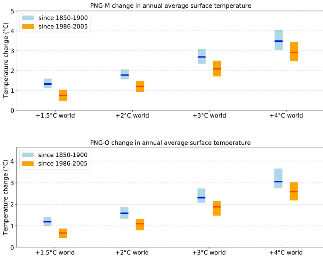
Figure 4.5. Change in the average annual temperature of the Papua New Guinea regions (M for Mainland, O for Ocean and Islands) at different global warming levels, from the 1850-1900 baseline, and from the more recent baseline of 1986-2005. The bars represent multi-model median and 10th-90th percentile range.
