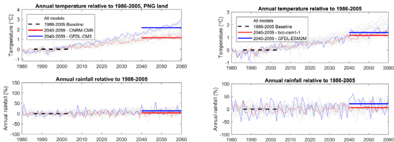
Figure 6.2 Modelled annual temperature (°C) and rainfall (%) changes in the Papua New Guinea Mainland (left) and Ocean and Islands (right) regions relative to 1986-2005 from CMIP5 models, showing the selected models that are representative of a warm dry future (red) and a hot wet future (blue).
