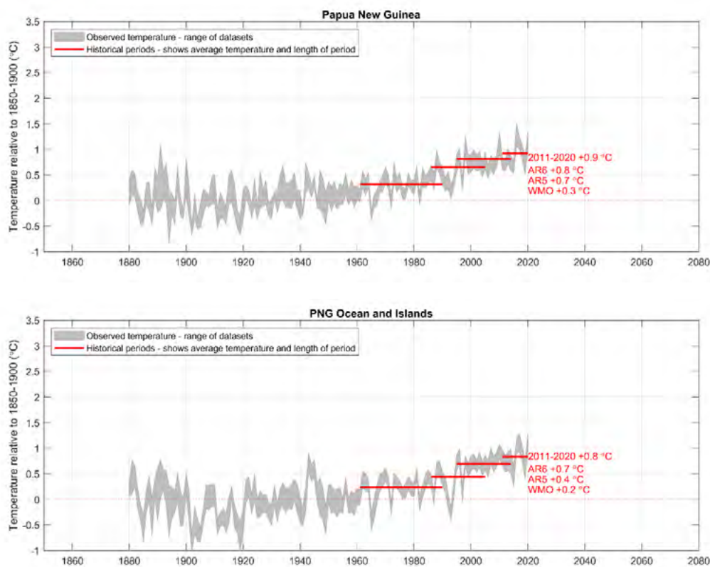
Figure 2.2 Average annual temperature of Papua New Guinea relative to 1850-1900 (°C; grey band indicates the range of five global temperature datasets) and the climate average for four different historical periods (baselines), as marked:
