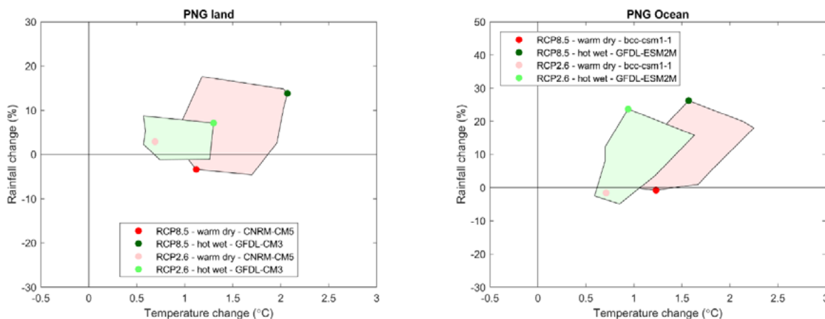
Figure 6.1 Modelled change in annual temperature and rainfall in the Papua New Guinea Mainland (left) and Ocean and Islands (right) regions between 1986-2005 and 2040-2059 from CMIP5 models (coloured shapes), showing the selected models that are representative of a warm dry future and a hot wet future for RCP2.6 (low case: green polygon) and RCP8.5 (high case: red polygon).
