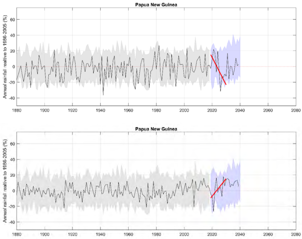
Figure 3.2 Mean annual rainfall of the Papua New Guinea Mainland region relative to 1986-2005 (%) from the group of CMIP5 models (grey band: historic, blue band: future), with an example model run shown in each panel (black line) highlighting the different possible trend in 2021-2030: (top) a model showing a decrease (red trend line), and (bottom) a model showing an increase.
