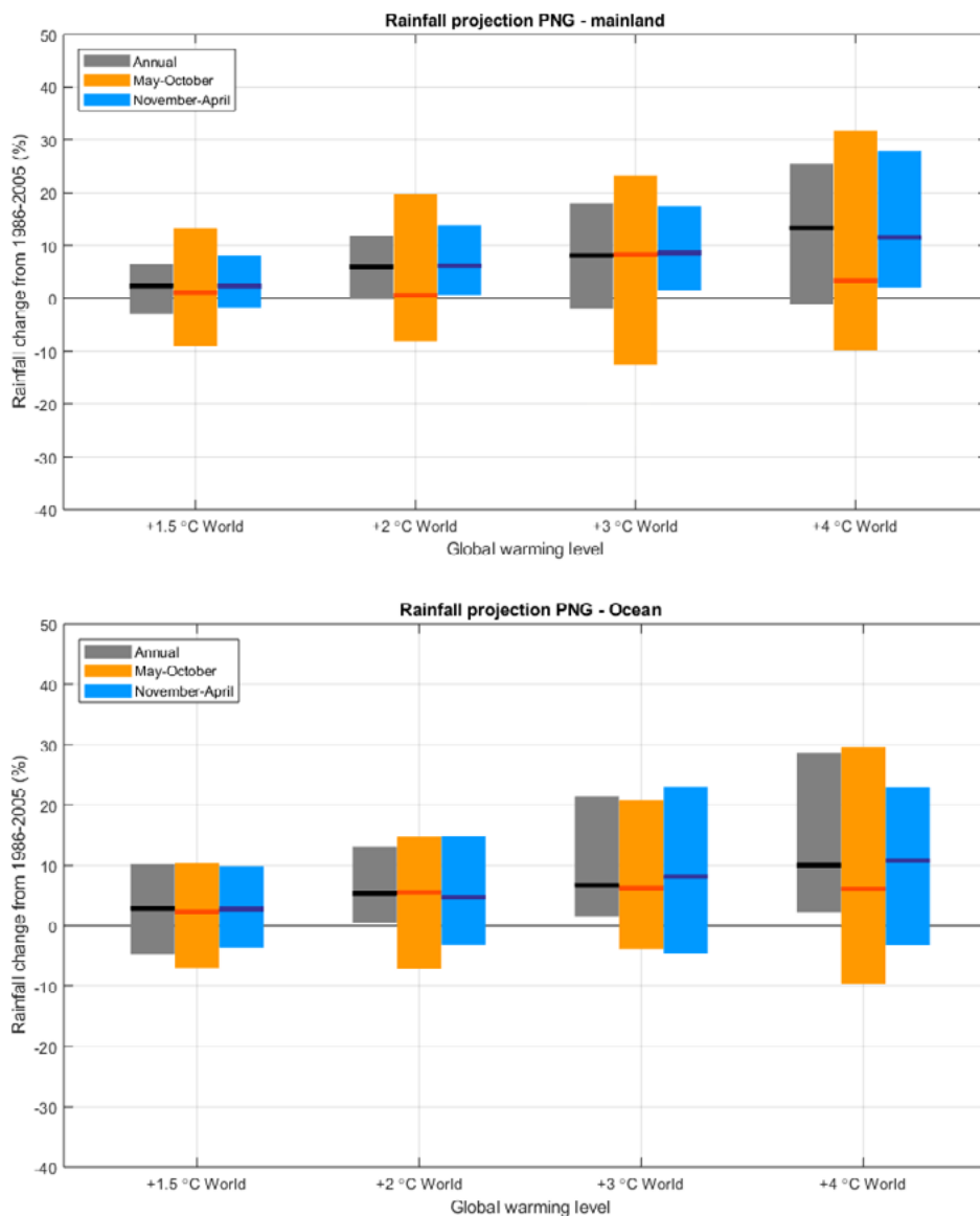
Figure 4.6. Change in the average annual and 6-month seasonal rainfall in the Papua New Guinea region at different global warming levels relative to the 1986-2005 baseline. The bars represent multi-model median and 10th-90th percentile range.
