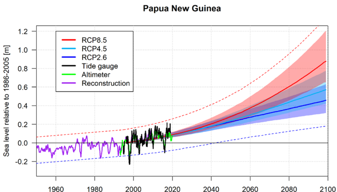
Figure 5.2 Sea level rise projections for Papua New Guinea. The tide gauge record of relative sea level at Lombrum is indicated in black, the satellite record in green and reconstructed sea level data is shown in purple, all are monthly means without seasonal cycles and referenced to mean sea level between 1986-2005. Multi-model-mean projections from 1995-2100 are given for the RCP8.5 (red solid line), RCP4.5 (cyan solid line) and RCP2.6 emissions scenarios (blue solid line), with the 5–95% uncertainty range for RCP8.5 and RCP2.6, shown by the red and blue shaded regions respectively. The dashed lines are an estimate of interannual variability in sea level (5–95% uncertainty range) and indicate that individual monthly averages of sea level can be above or below longer-term averages.
