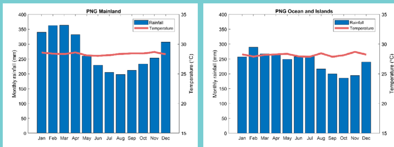
Figure 1.2. Mean annual cycle of rainfall and temperature in Papua New Guinea in 1981-2010 (rainfall uses ERA5, temperature uses HadCRUT5, see Methods in Section 8).
