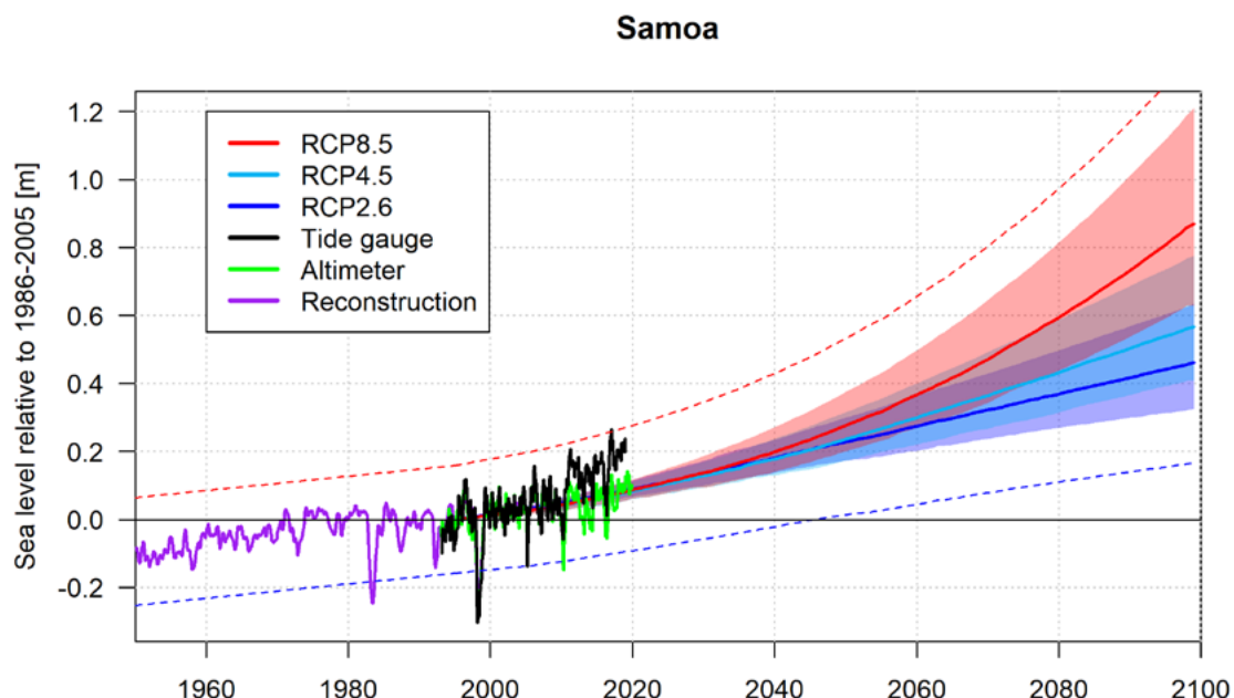
Figure 5.2 Sea level rise projections for Samoa. The tide gauge record of relative sea level at Apia is indicated in black, the satellite record in green and reconstructed sea level data is shown in purple, all are monthly means without seasonal cycles and referenced to mean sea level between 1986–2005 (note that the departure between the tide gauge and altimeter since 2009 is likely due to land subsidence after the 2009 earthquake). Multi-model-mean projections from 1995–2100 are given for the RCP8.5 (red solid line), RCP4.5 (cyan solid line) and RCP2.6 emissions scenarios (blue solid line), with the 5–95% uncertainty range for RCP8.5 and RCP2.6 shown by the red and blue shaded regions respectively. The dashed lines are an estimate of interannual variability in sea level (5–95% uncertainty range) and indicate that individual monthly averages of sea level can be above or below longer-term averages.
