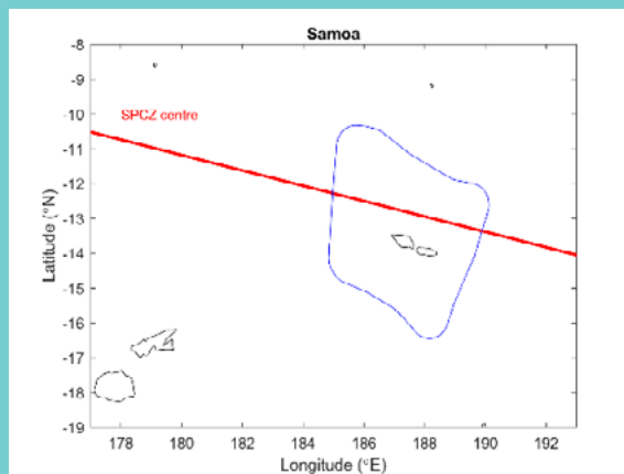
Figure 1.1. Map of Samoa (top) and the mask area (centre) for calculating areal averages from gridded observational data and climate models' outputs.
