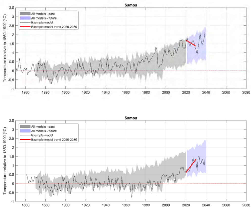
Figure 2.5. Average annual temperature in Samoa relative to 1850-1900 (°C) simulated in CMIP5 models, showing the range of all models (historic; grey band, future; blue band) and example model simulations (black line) with the linear trend for 2020-2030 marked (red line); top: an example with suppressed warming in 2020-2030 due to climate variability, bottom: an example where variability enhances the warming trend in 2020-2030.
