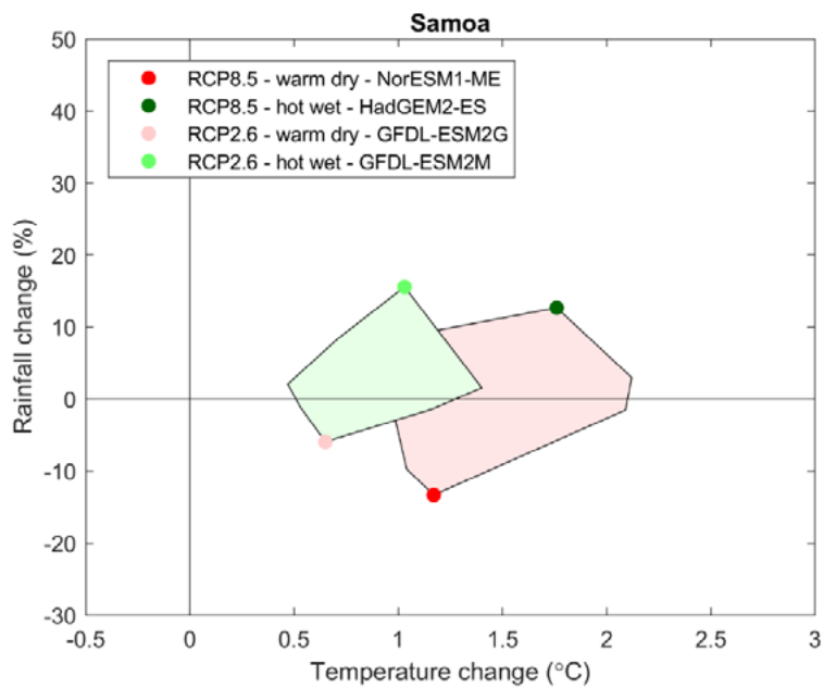
Figure 6.1 Modelled change in annual temperature and rainfall between 1986-2005 and 2040-2059 from CMIP5 models (coloured shapes) in the Samoa region, showing the selected models that are representative of a warm dry future and a hot wet future for RCP2.6 (low case: green polygon) and RCP8.5 (high case: red polygon).
