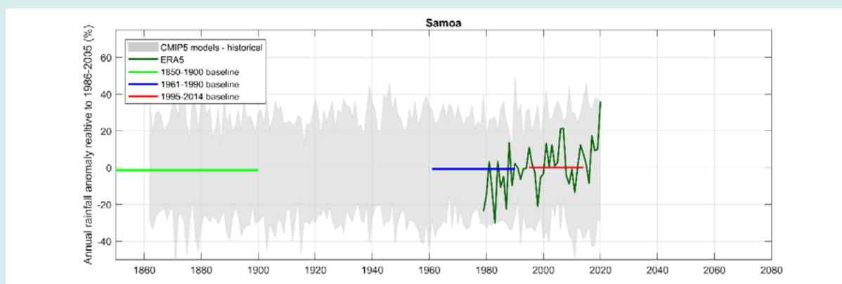
Figure 3.1 Area-average of Samoa region annual rainfall (%) relative to the 1986-2005 period from gridded observations (ERA5 shown, results are similar from GPCP, CMAP and ERA5), the range of CMIP5 models (grey band). Coloured horizontal bars show the average of all models for the baseline periods described in the legend.
