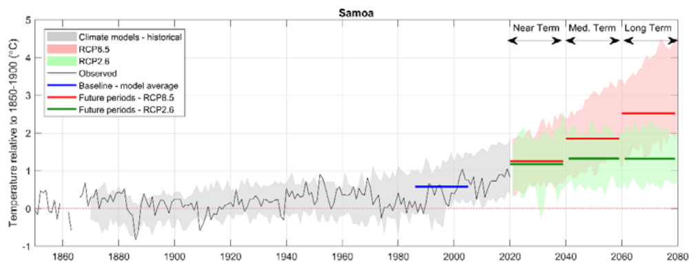
Figure 2.6. Average annual temperature in Samoa region relative to 1850-1900 (°C) derived from observations (Berkeley shown; grey solid line) and simulated in CMIP5 models, showing the range of all models for the past period (grey band), the future under a very high emissions pathway (pink band) and a very low emissions pathway (green band). Thick horizontal lines show the mean of all models in 20-year periods of the baseline 1986-2005 (blue) and future 20-year periods centred on 2030, 2050 and 2070 (RCP8.5; red horizontal lines, RCP2.6; green horizontal lines).
