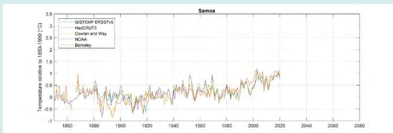
Figure 2.1. Average annual temperature of the Samoa region relative to 1850-1900 in five global datasets (see Methods, Section 8 for details).
