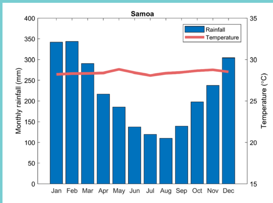
Figure 1.2. Mean annual cycle of rainfall and temperature in Samoa in 1981-2010 (rainfall uses ERA5, temperature uses HadCRUT5, see Methods in Section 8).
