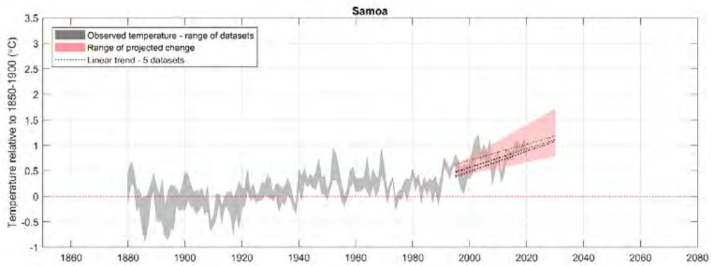
Figure 2.4 Average annual temperature of the Samoa region relative to 1850-1900 (°C; grey band indicates range of five global temperature datasets), the reported range of projected change from PACCSAP is shown as a red wedge (the starting point allows for the difference between the five datasets) and the linear trend of smoothed observations for 1995-2020 plotted and extrapolated forward to 2030 (one dotted line for each dataset).
