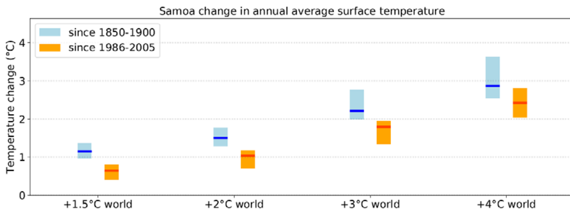
Figure 4.5. Change in the average annual temperature of the Samoa region at different global warming levels, from the 1850-1900 baseline, and from the more recent baseline of 1986-2005. The bars represent multi-model median and 10th-90th percentile range.
