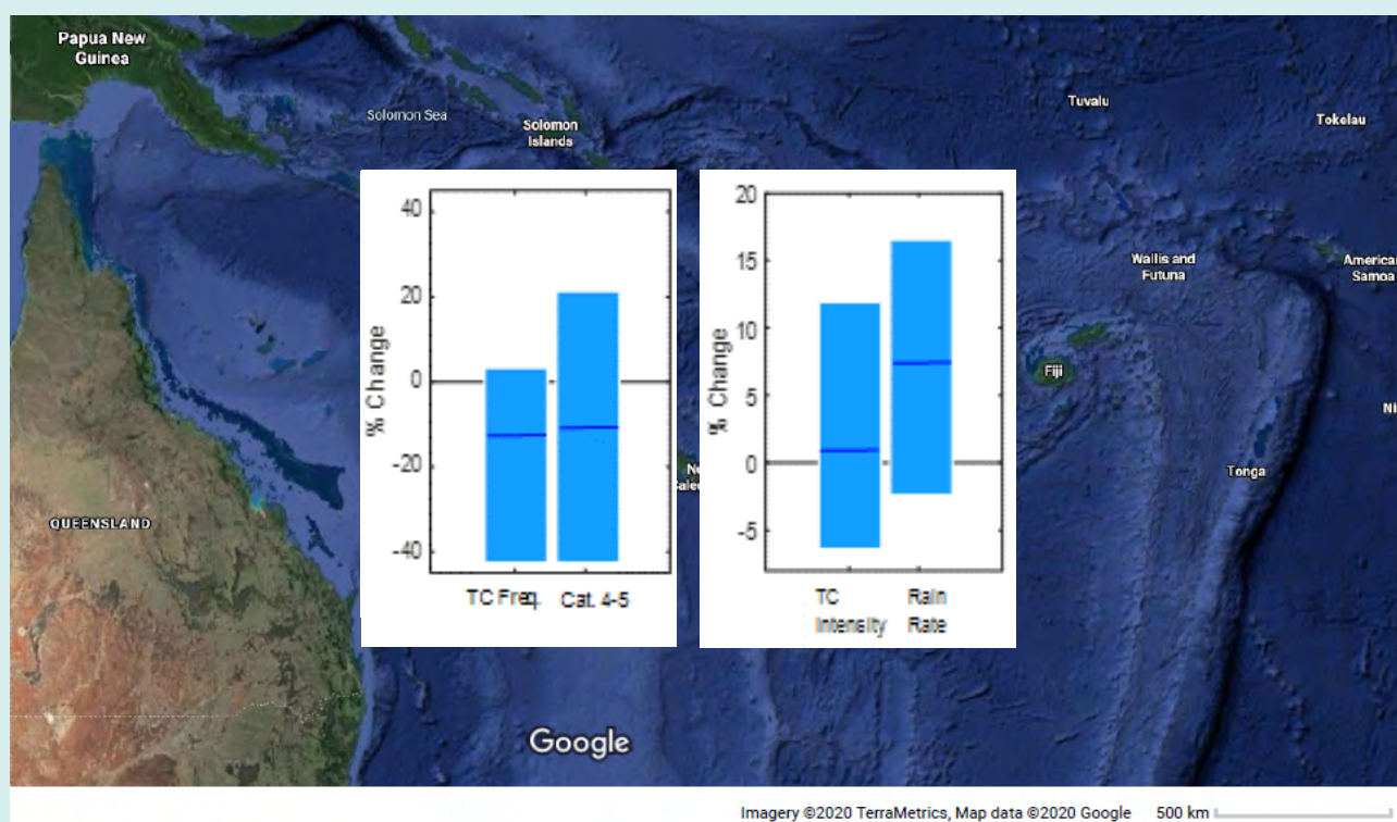
Figure 5.1 Southwest Pacific TC activity projection for a 2°C global warming. The bars on the left indicate a likely decrease in the total number of TCs, and a likely decrease but possible increase in severe (category 4-5) TCs. Bars on the right plot indicate a likely increase (but possible decrease) in the average intensity of TCs, and the very likely increase in the rainfall they bring. Shown are the median (blue line) and the 10th–90th-percentile ranges (blue bars). (Information used to construct this figure is derived from Knutson et al. 2020).
