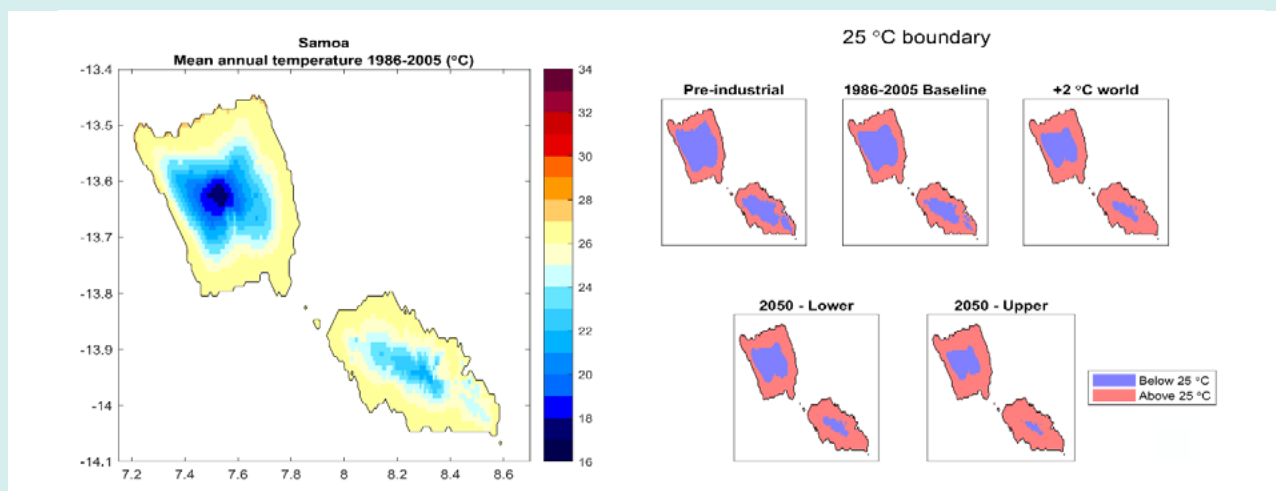
Figure 7.1. The average annual temperature in 1986-2005 in Samoa (left: the 'WorldClim' high-resolution climate surface adjusted for the baseline used), and the area of the island above or below the 25°C boundary for various scenarios (right).
