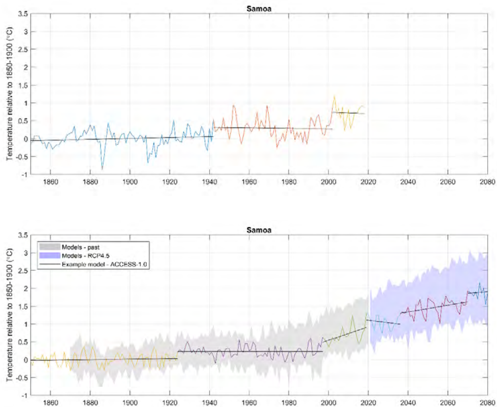
Figure 2.7. Annual average temperature of Samoa relative to the 1850-1900 (°C) baseline showing detected eras separated by breakpoints (see Data and Methods): top: in observations (Cowtan and Way 2014) showing three eras, early in the time series (blue), then ‘jump’ to a warmer period through mid to late 20th Century (orange), and the warmer 2000s (yellow); and bottom: an example model simulation, showing step-like changes throughout the past and future. Example model simulation is from ACCESS-1.0 under moderate emissions RCP4.5 (results are similar but with lower background warming in RCP2.6, and higher background warming in RCP8.5).
