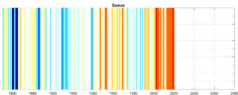
Figure 2.3 Samoa region temperature relative to 1961-1990 through time presented as ‘climate stripes’ devised by Hawkins (2018): red = hotter, blue = cooler (using the Berkeley dataset).
