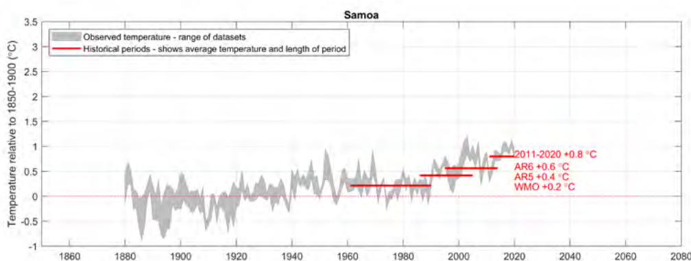
Figure 2.2 Average annual temperature of Samoa region relative to 1850-1900 (°C; grey band indicates the range of five global temperature datasets) and the climate average for four different historical periods (baselines), as marked:
