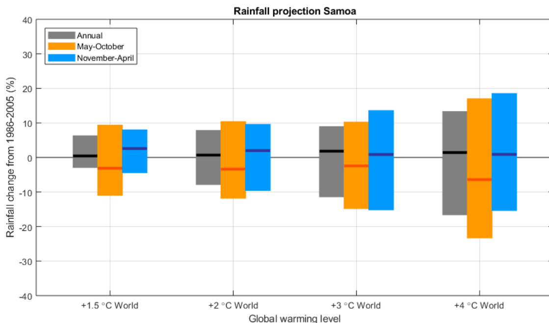
Figure 4.6. Change in the average annual and 6-month seasonal rainfall in the Samoa region at different global warming levels relative to the 1986-2005 baseline. The bars represent multi-model median and 10th-90th percentile range.
