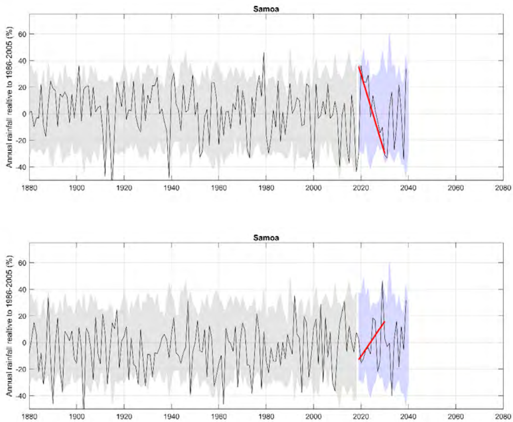
Figure 3.2 Mean annual rainfall of the Samoa region relative to 1986-2005 (%) from the group of CMIP5 models (grey band: historic, blue band: future), with an example model run shown in each panel (black line) highlighting the different possible trend in 2021-2030: (top) a model showing a decrease (red trend line in the top panel), and (bottom) a model showing an increase (red trend line in the bottom panel).
