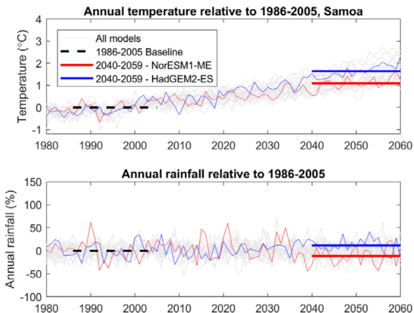
Figure 6.2 Modelled annual temperature (°C) and rainfall (%) changes relative to 1986-2005 from CMIP5 models in the Samoa region, showing the selected models that are representative of a warm dry future (red) and a hot wet future (blue) for RCP8.5 (High Case).
