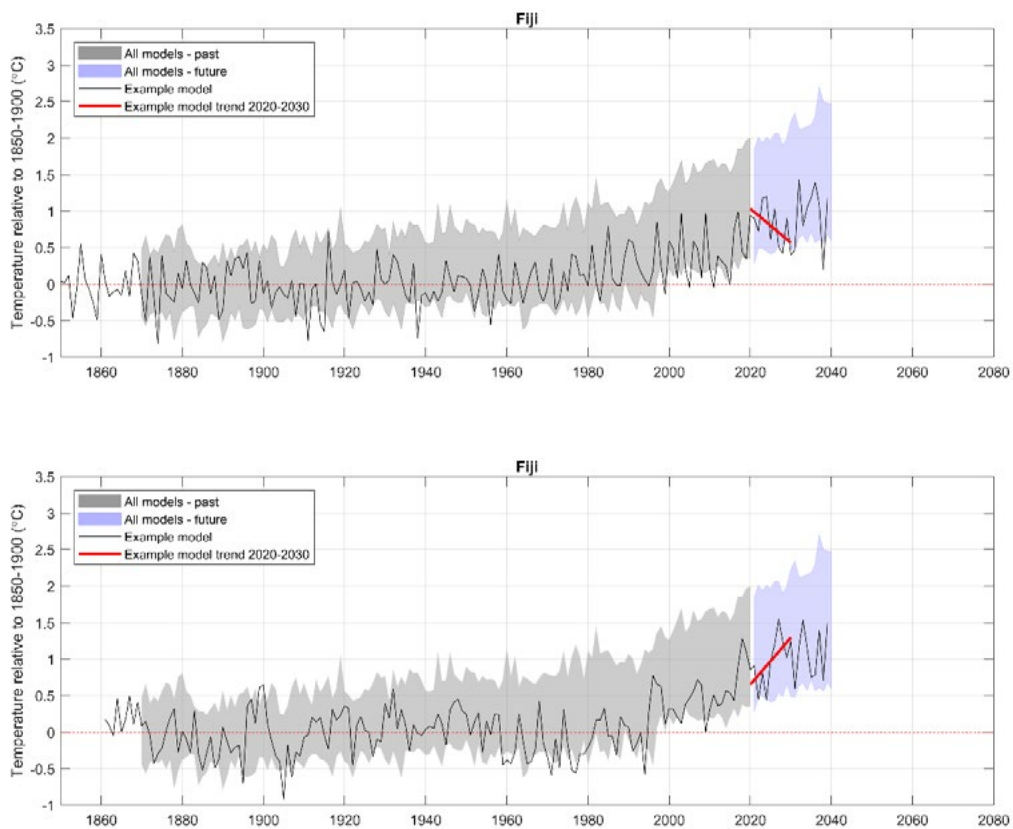
Figure 2.5. Average annual temperature in Fiji relative to 1850-1900 (°C) simulated in CMIP5 models, showing the range of all models (historic; grey band, future; blue band) and example model simulations (black line) with the linear trend for 2020-2030 marked (red line); top: an example with suppressed warming in 2020-2030 due to climate variability, bottom: an example where variability enhances the warming trend in 2020-2030.
