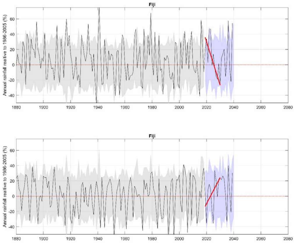
Figure 3.2 Mean annual rainfall of the Fiji region relative to 1986-2005 (%) from the group of CMIP5 models (grey band: historic, blue band: future), with an example model run shown in each panel (black line) highlighting the different possible trend in 2021-2030: (top) a model showing a decrease (red trend line in the top panel), and (bottom) a model showing an increase (red trend line in the bottom panel).
