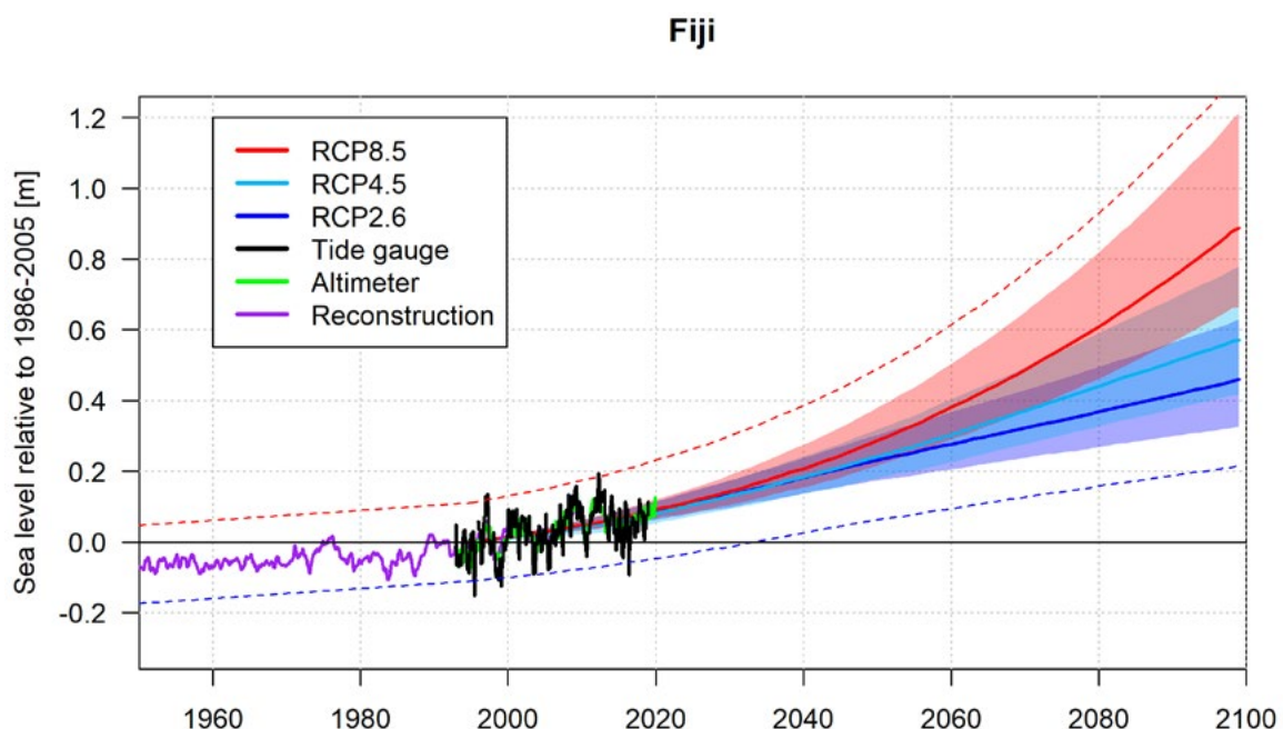
Figure 5.2 Sea level rise projections for Fiji. The tide gauge record of relative sea level at Lautoka is indicated in black, the satellite record in green and reconstructed sea level data is shown in purple, all are monthly means without seasonal cycles and referenced to mean sea level between 1986-2005. Multi-model-mean projections from 1995-2100 are given for the RCP8.5 (red solid line), RCP4.5 (cyan solid line) and RCP2.6 emissions scenarios (blue solid line), with the 5–95% uncertainty range for RCP8.5 and RCP2.6 shown by the red and blue shaded regions respectively. The dashed lines are an estimate of interannual variability in sea level (5–95% uncertainty range and indicate that individual monthly averages of sea level can be above or below longer-term averages).
