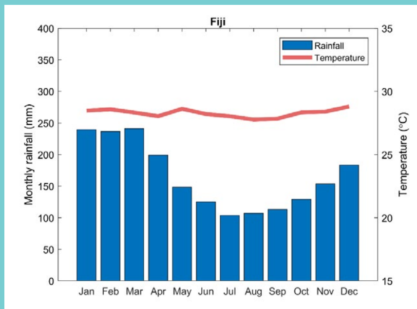
Figure 1.2. Mean annual cycle of rainfall and temperature in Fiji in 1981-2010 (rainfall uses ERA5, temperature uses HadCRUT5, see Methods in Section 8).
