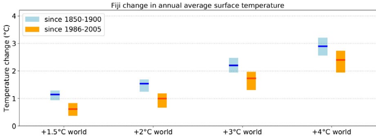
Figure 4.5. Change in the average annual temperature of the Fiji region at different global warming levels, from the 1850-1900 baseline, and from the more recent baseline of 1986-2005. The bars represent multi-model median and 10th-90th percentile range.
