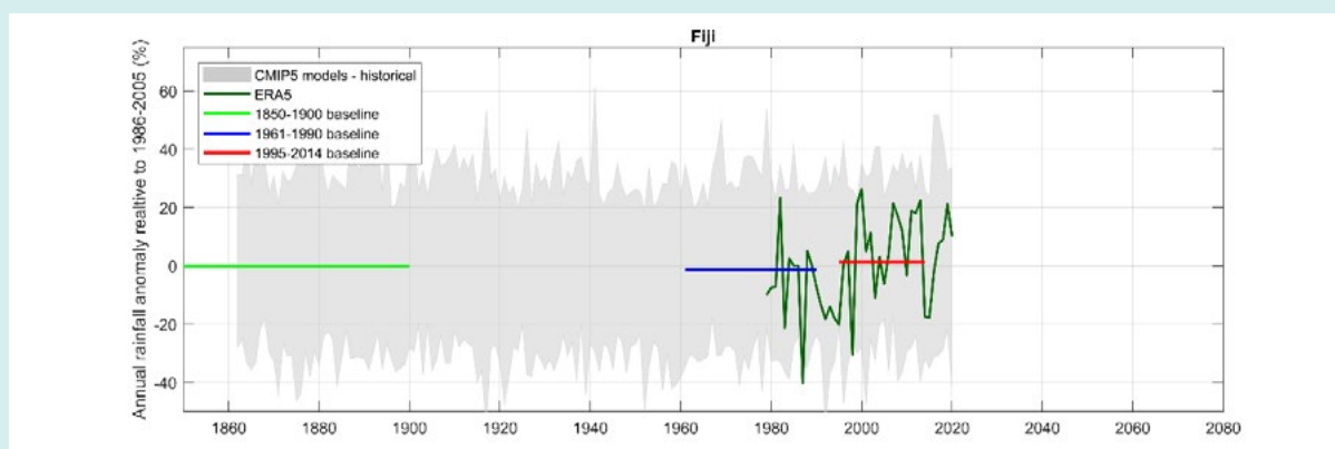
Figure 3.1 Area-average of Fiji annual rainfall (%) relative to the 1986-2005 period from gridded observations (ERA5 shown, results are similar from GPCP, CMAP and ERA5), the range of CMIP5 models (grey band). Coloured horizontal bars show the average of all models for the baseline periods described in the legend.
