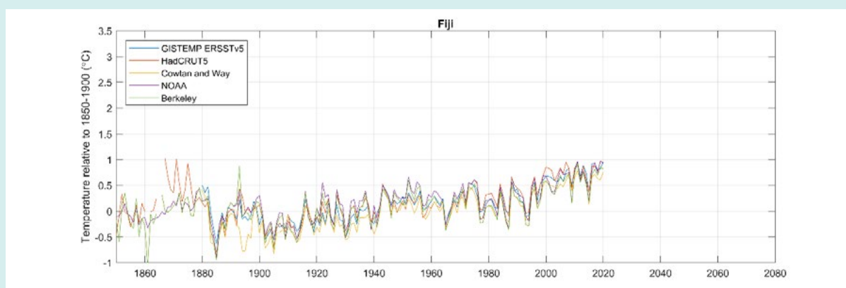
Figure 2.1. Average annual temperature of the Fiji region relative to 1850-1900 in five global datasets (see Methods, Section 8 for details).
