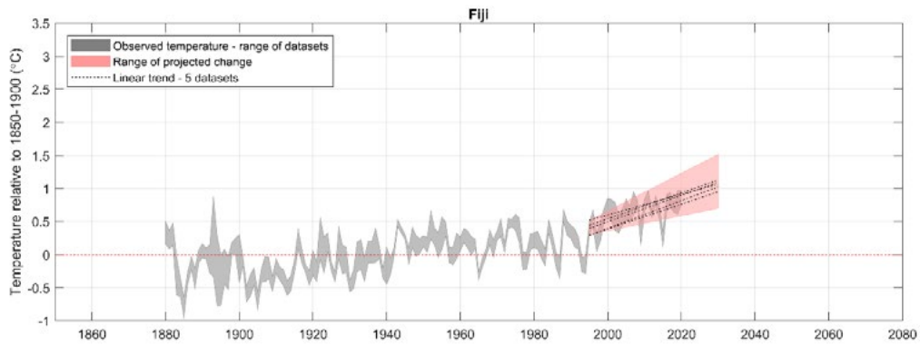
Figure 2.4 Average annual temperature of the Fiji region relative to 1850-1900 (°C; grey band indicates range of five global temperature datasets), the reported range of projected change from PACCSAP is shown as a red wedge (the starting point allows for the difference between the five datasets) and the linear trend of smoothed observations for 1995-2020 plotted and extrapolated forward to 2030 (one dotted line for each dataset).
