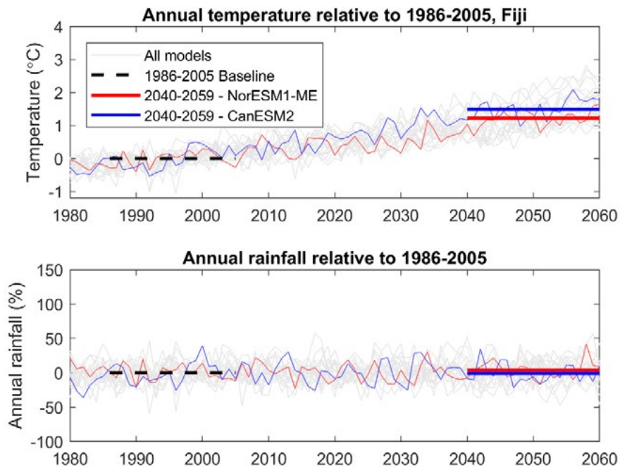
Figure 6.2 Modelled annual temperature (°C) and rainfall (%) changes in the Fiji region relative to 1986-2005 from CMIP5 models, showing the selected models that are representative of a warm dry future (NorESM1-ME, red) and a hot wet future (CanESM2, blue).
