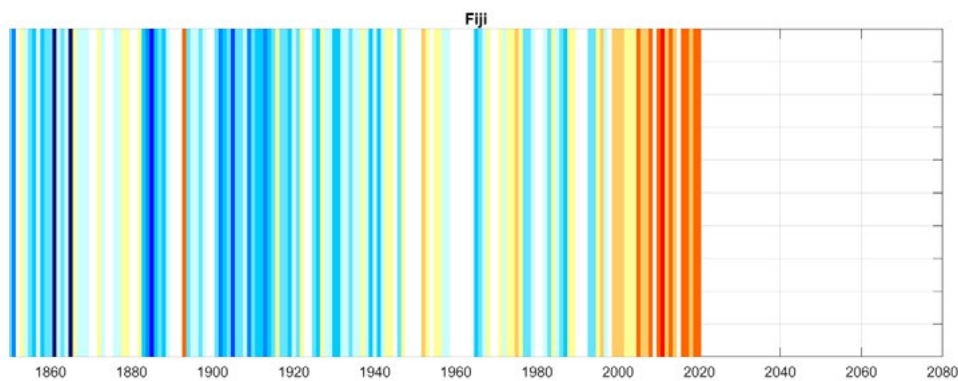
Figure 2.3 Fiji temperature relative to 1961-1990 through time presented as ‘climate stripes’ devised by Hawkins (2018): red = hotter, blue = cooler (using the Berkeley dataset).
