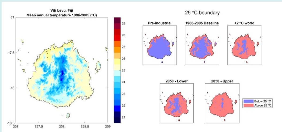
Figure 7.1. The average annual temperature in 1986-2005 in Viti Levu (left: the 'WorldClim' high-resolution climate surface adjusted for the baseline used), and the area of the island above or below the 25°C boundary for various scenarios (right).
