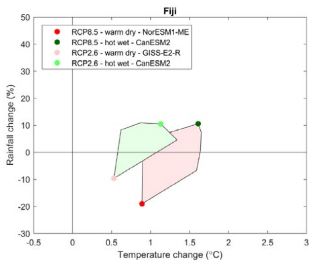
Figure 6.1 Modelled change in annual temperature and rainfall in the Fiji region between 1986-2005 and 2040-2059 from CMIP5 models (coloured shapes), showing the selected models that are representative of a warm dry future and a hot wet future for RCP2.6 (low case: green polygon) and RCP8.5 (high case: red polygon).
