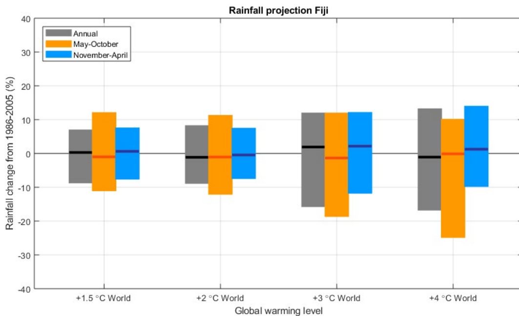
Figure 4.6. Change in the average annual and 6-month seasonal rainfall in the Fiji region at different global warming levels relative to the 1986-2005 baseline. The bars represent multi-model median and 10th-90th percentile range.
