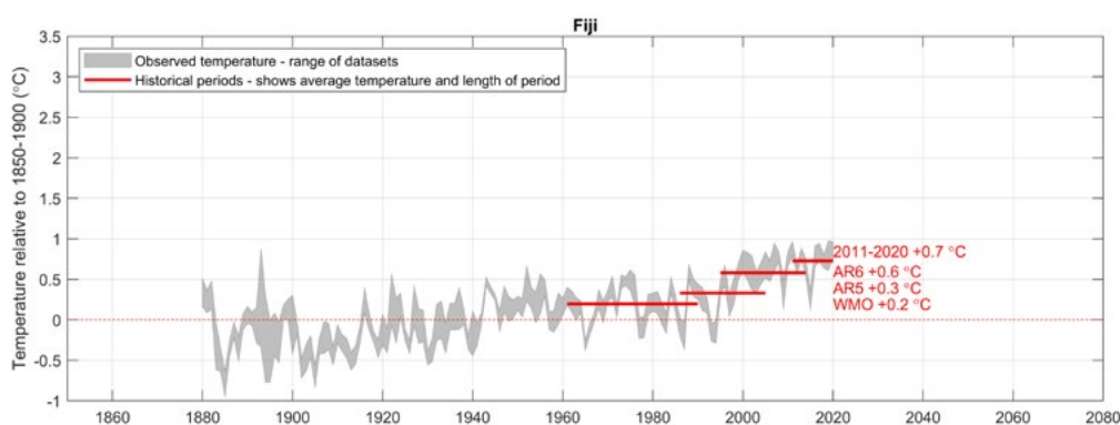
Figure 2.2 Average annual temperature of Fiji relative to 1850-1900 (°C; grey band indicates the range of five global temperature datasets) and the climate average for four different historical periods (baselines), as marked:
