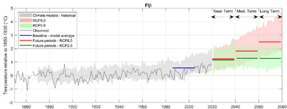
Figure 2.6. Average annual temperature in Fiji relative to 1850-1900 (°C) derived from observations (Berkeley shown; grey solid line) and simulated in CMIP5 models, showing the range of all models for the past period (grey band), the future under a very high emissions pathway (pink band) and a very low emissions pathway (green band). Thick horizontal lines show the mean of all models in 20-year periods of the baseline 1986-2005 (blue) and future 20-year periods centred on 2030, 2050 and 2070 (RCP8.5; red horizontal lines, RCP2.6; green horizontal lines).
