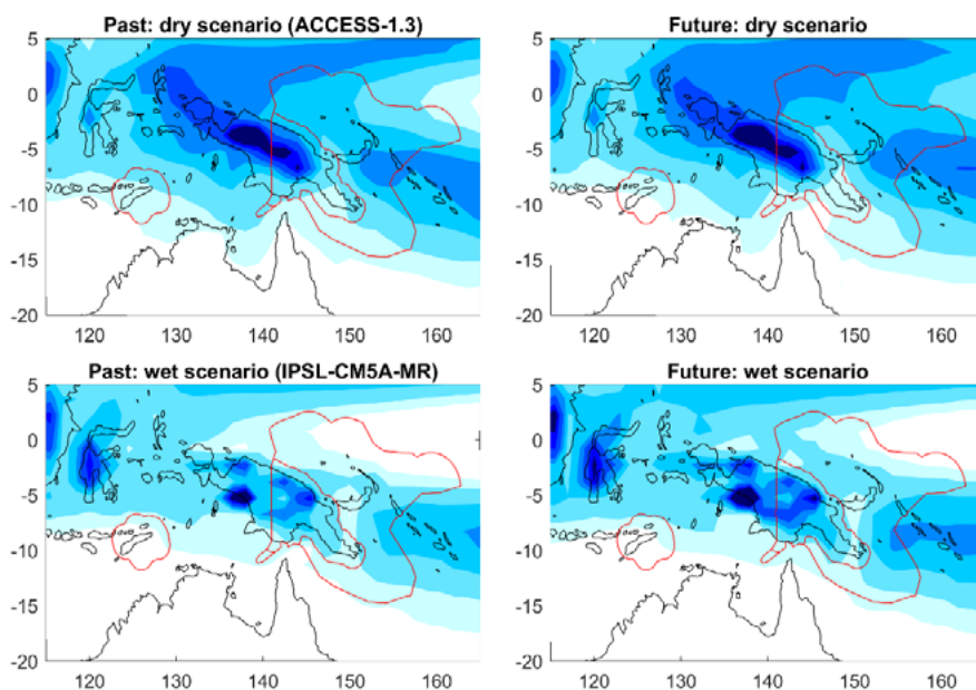
Figure 6.3 The mean annual rainfall of the Asia-Australian monsoon region (bluer is wetter) in the 1986-2005 (past) and the 2040-2059 (future) periods as simulated in the models used to represent the warm and dry scenario (top) and the hot and wet scenario (bottom).
