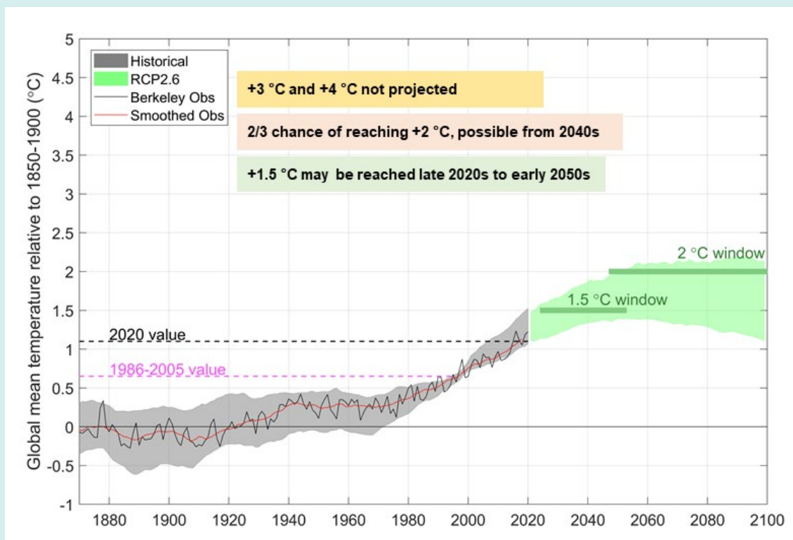
Figure 4.1 Global average surface temperature relative to 1850-1900 in Berkeley observations (grey line: annual value, red line: 41-year Lowess smoother), in the CMIP5 models for historical (grey band) and future under RCP2.6 (green band). The rough time window when global warming levels could be reached is shown by dark horizontal bars. Note models are calibrated relative to the 1986-2005 baseline and the observed change between 1850-1900 and 1986-2005 is added.
