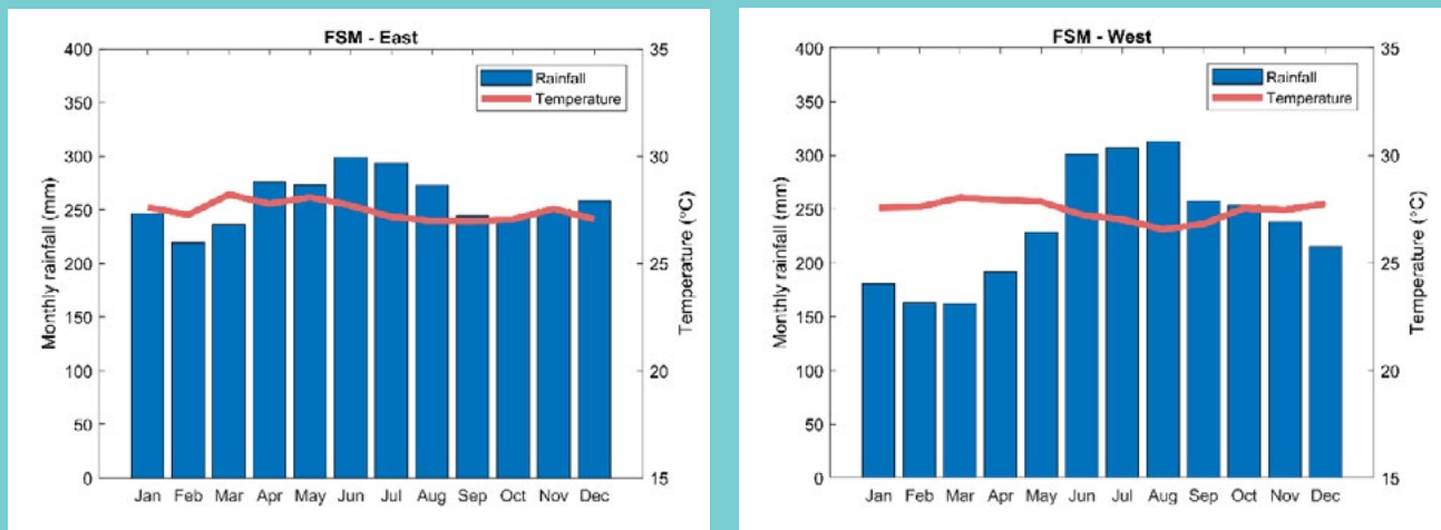
Figure 1.2. Mean annual cycle of rainfall and temperature in FSM in 1981-2010 (rainfall uses ERA5, temperature uses HadCRUT5, see Methods in Section 8).
