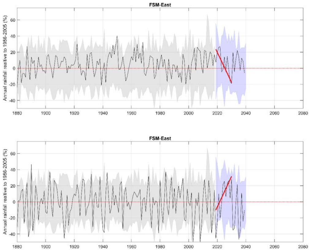
Figure 3.2 Mean annual rainfall of the FSM region relative to 1986-2005 (%) from the group of CMIP5 models (grey band: historic, blue band: future), with an example model run shown in each panel (black line) highlighting the different possible trend in 2021-2030: (top) a model showing a decrease (red trend line in the top panel), and (bottom) a model showing an increase (red trend line in the bottom panel).
