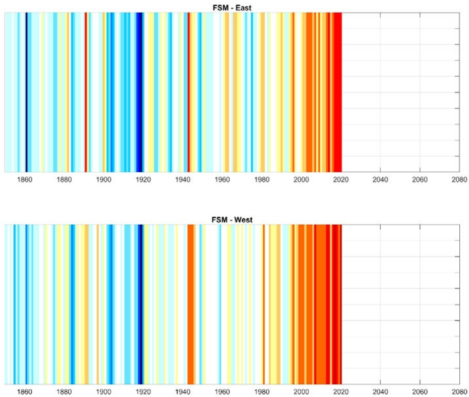
Figure 2.3 FSM east and west temperature relative to 1961-1990 through time presented as 'climate stripes' devised by Hawkins (2018): red = hotter, blue = cooler (using the Berkeley dataset).
