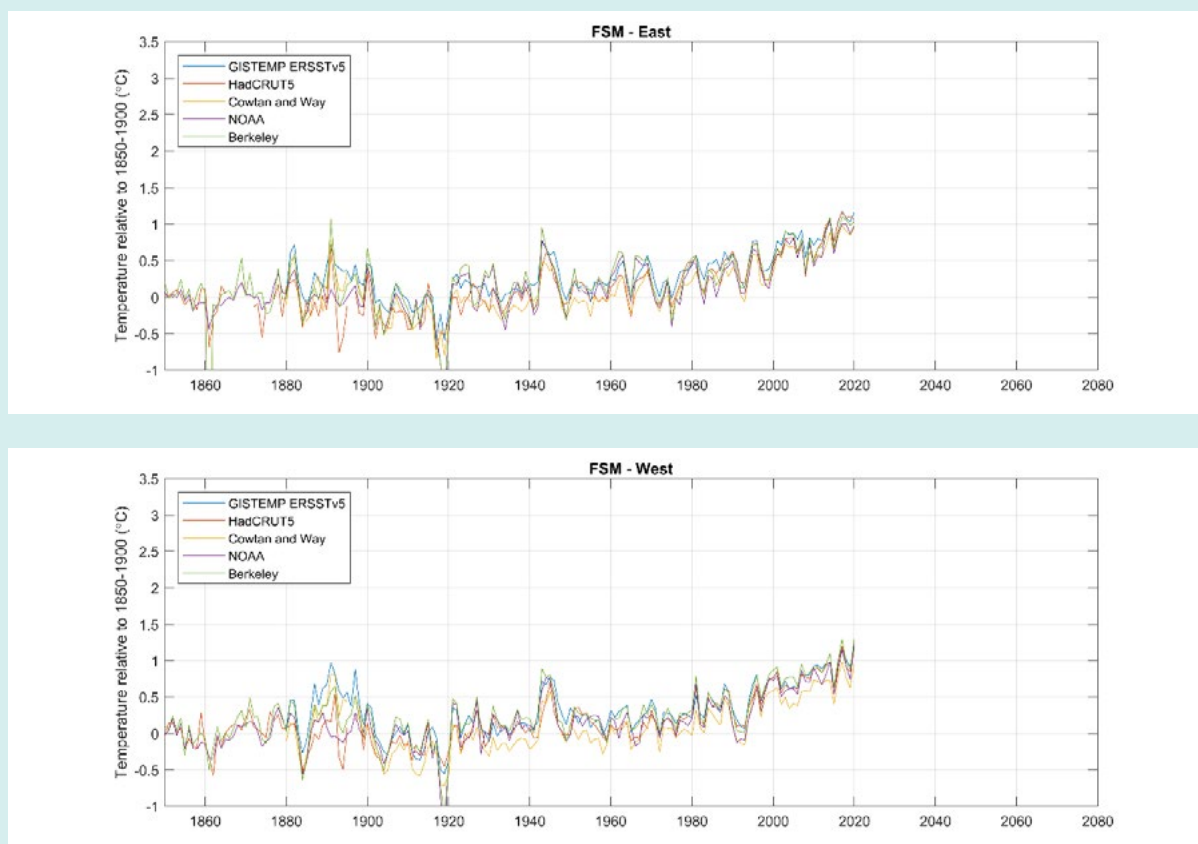
Figure 2.1. Average annual temperature of FSM east and west relative to 1850-1900 in five global datasets (see Methods, Section 8 for details).
