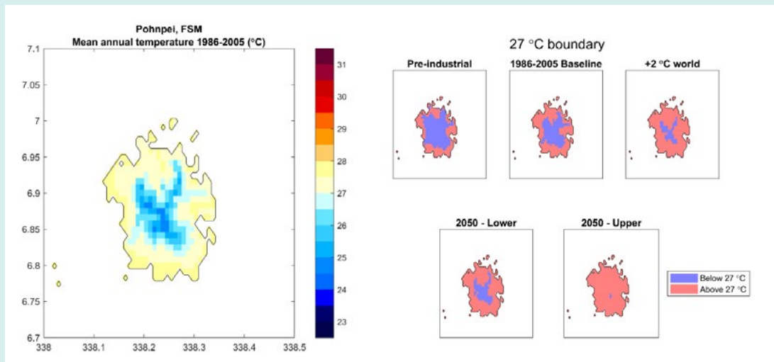
Figure 7.1. The average annual temperature in 1986-2005 in Pohnpei (left: the 'WorldClim' high-resolution climate surface adjusted for the baseline used), and the area of the island above or below the 27°C boundary for various scenarios (right).
