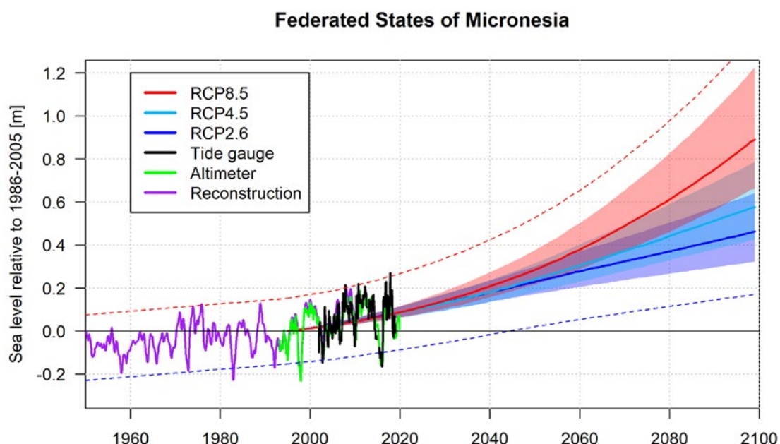
Figure 5.2 Sea level rise projections for Federated States of Micronesia. The tide gauge record of relative sea level at Pohnpei is indicated in black, the satellite record in green and reconstructed sea level data is shown in purple, all are monthly means without seasonal cycles and referenced to mean sea level between 1986-2005. Multi-model-mean projections from 1995–2100 are given for the RCP8.5 (red solid line), RCP4.5 (cyan solid line) and RCP2.6 emissions scenarios (blue solid line), with the 5–95% uncertainty range for RCP8.5 and RCP2.6 shown by the red and blue shaded regions respectively. The dashed lines are an estimate of interannual variability in sea level (5–95% uncertainty range) and indicate that individual monthly averages of sea level can be above or below longer-term averages.
