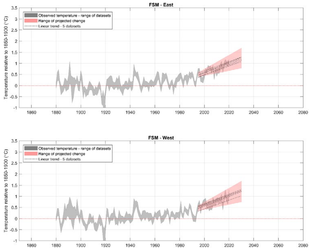
Figure 2.4 Average annual temperature of the FSM east and west regions relative to 1850-1900 (°C; grey band indicates range of five global temperature datasets), the reported range of projected change from PACCSAP is shown as a red wedge (the starting point allows for the difference between the five datasets) and the linear trend of smoothed observations for 1995-2020 plotted and extrapolated forward to 2030 (one dotted line for each dataset).
