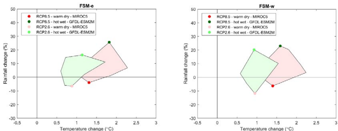
Figure 6.1 Modelled change in annual temperature and rainfall in the FSM region between 1986-2005 and 2040-2059 from CMIP5 models (coloured shapes), showing the selected models that are representative of a warm dry future and a hot wet future for RCP2.6 (low case: green polygon) and RCP8.5 (high case: red polygon).
