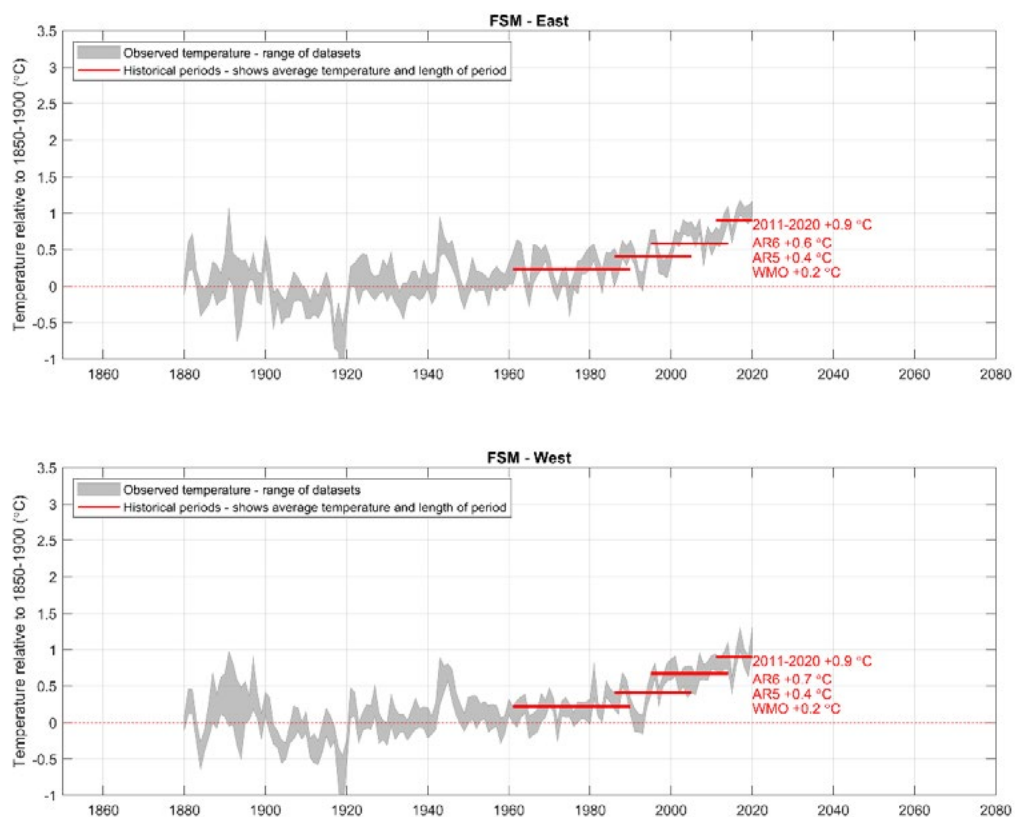
Figure 2.2 Average annual temperature of FSM east and west relative to 1850-1900 (°C; grey band indicates the range of five global temperature datasets) and the climate average for four different historical periods (baselines), as marked:
