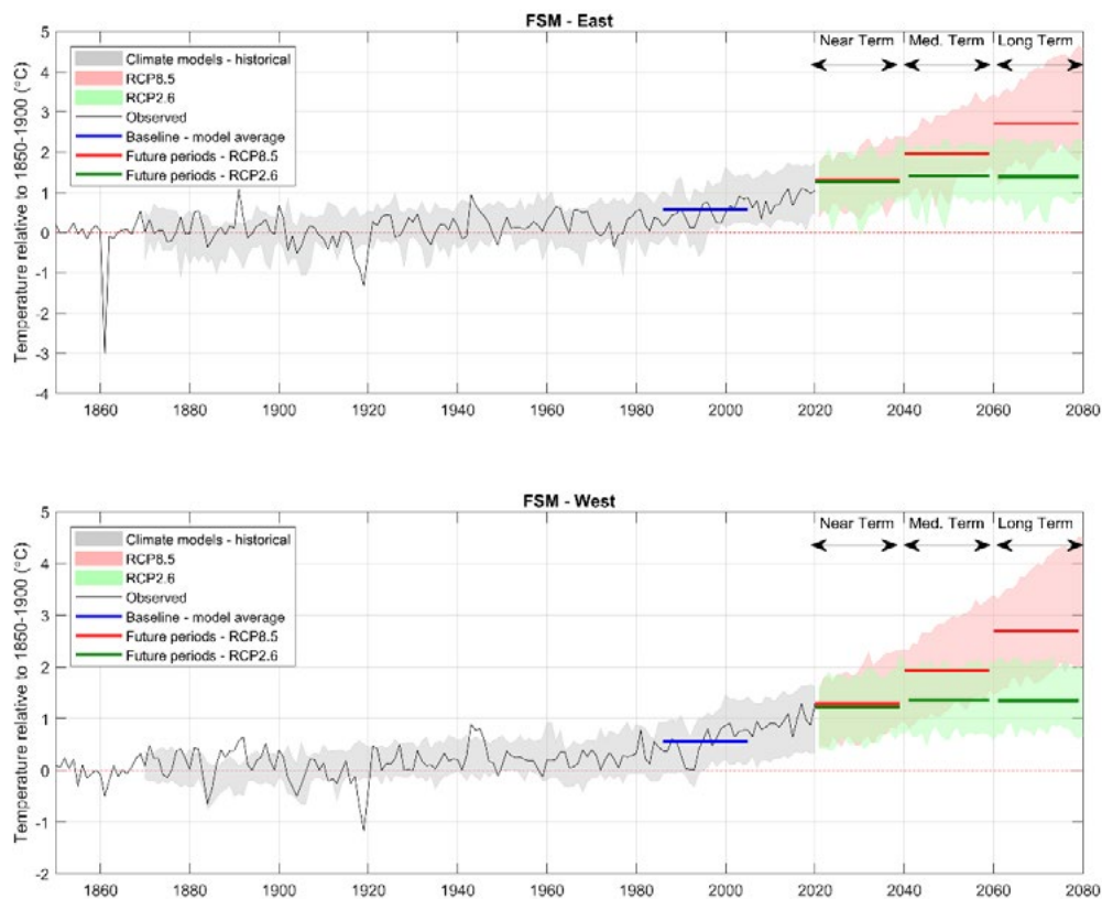
Figure 2.6. Average annual temperature in FSM east and west relative to 1850-1900 (°C) derived from observations (Berkeley shown; grey solid line) and simulated in CMIP5 models, showing the range of all models for the past period (grey band), the future under a very high emissions pathway (pink band) and a very low emissions pathway (green band). Thick horizontal lines show the mean of all models in 20-year periods of the baseline 1986-2005 (blue) and future 20-year periods centred on 2030, 2050 and 2070 (RCP8.5; red horizontal lines, RCP2.6; green horizontal lines).
