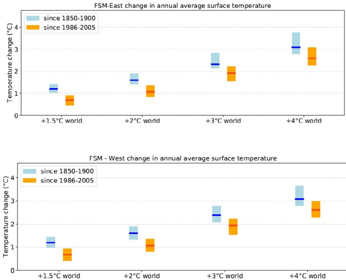
Figure 4.5. Change in the average annual temperature of FSM east and west at different global warming levels, from the 1850-1900 baseline, and from the more recent baseline of 1986-2005. The bars represent multi-model median and 10th-90th percentile range.
