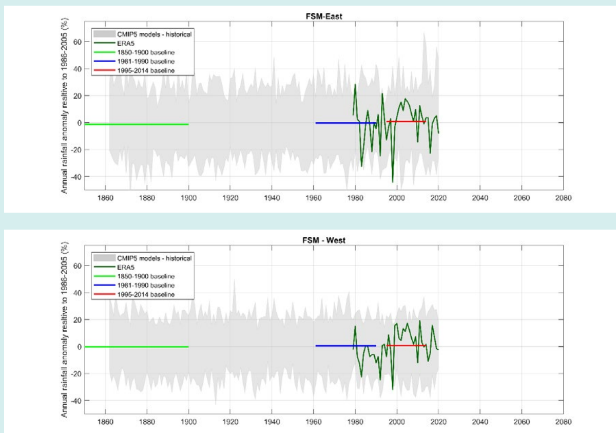
Figure 3.1 Area-average of FSM east and west annual rainfall (%) relative to the 1986-2005 period from gridded observations (ERA5 shown, results are similar from GPCP, CMAP and ERA5), the range of CMIP5 models (grey band). Coloured horizontal bars show the average of all models for the baseline periods described in the legend.
