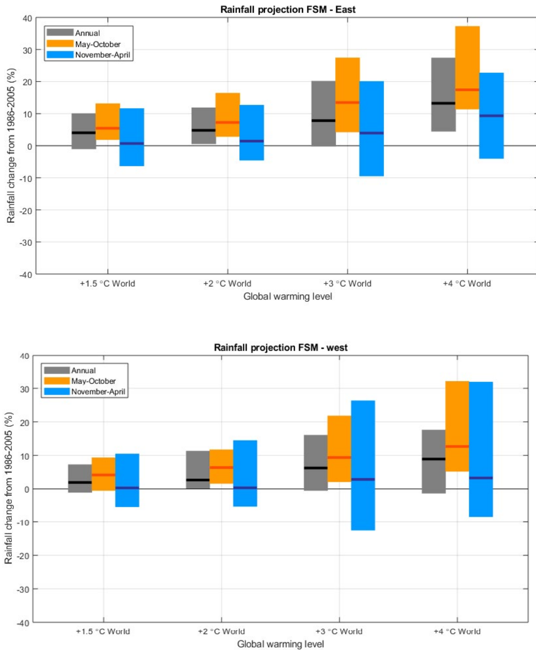
Figure 4.6. Change in the average annual and 6-month seasonal rainfall in the FSM region at different global warming levels relative to the 1986-2005 baseline. The bars represent multi-model median and 10th-90th percentile range.
