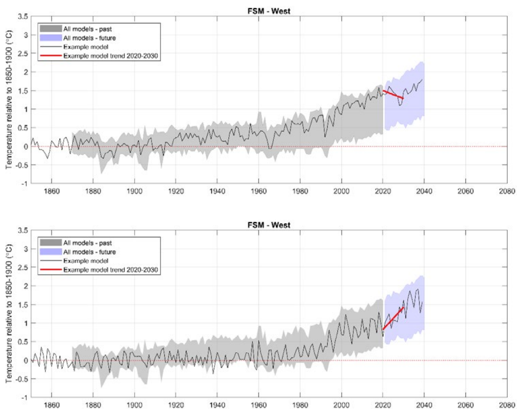
Figure 2.5. Average annual temperature in FSM west relative to 1850-1900 (°C) simulated in CMIP5 models, showing the range of all models (historic; grey band, future; blue band) and example model simulations (black line) with the linear trend for 2020-2030 marked (red line); top: an example with suppressed warming in 2020-2030 due to climate variability, bottom: an example where variability enhances the warming trend in 2020-2030.
