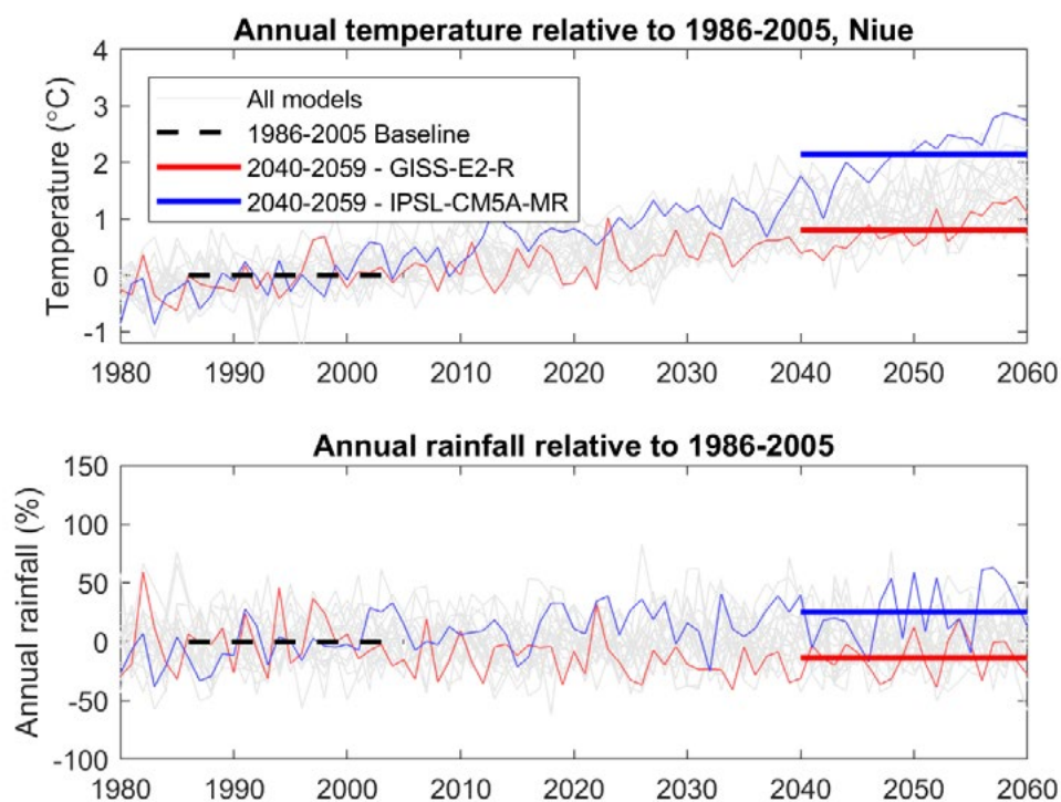
Figure 6.2 Modelled annual temperature (°C) and rainfall (%) changes in the Niue region relative to 1986-2005 from CMIP5 models, showing the selected models that are representative of a warm dry future (red) and a hot wet future (blue).
