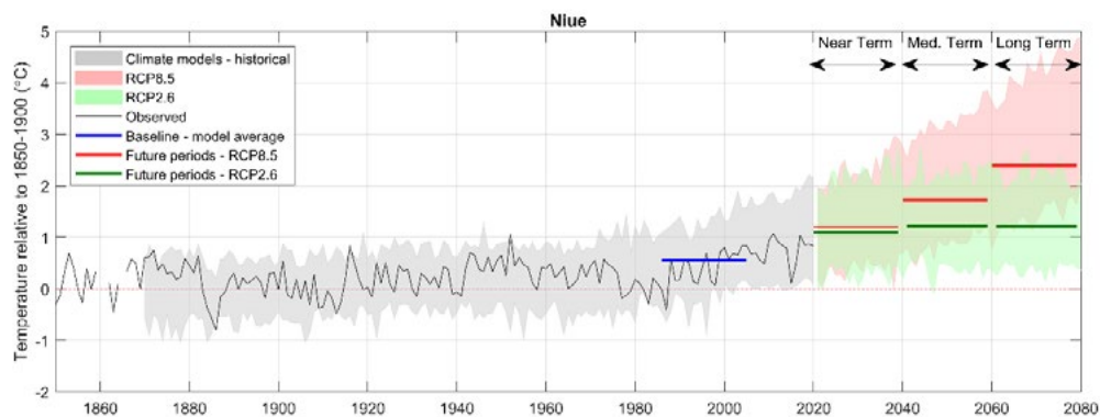
Figure 2.6. Average annual temperature in Niue relative to 1850-1900 (°C) derived from observations (Berkeley shown; grey solid line) and simulated in CMIP5 models, showing the range of all models for the past period (grey band), the future under a very high emissions pathway (pink band) and a very low emissions pathway (green band). Thick horizontal lines show the mean of all models in 20-year periods of the baseline 1986-2005 (blue) and future 20-year periods centred on 2030, 2050 and 2070 (RCP8.5; red horizontal lines, RCP2.6; green horizontal lines).
