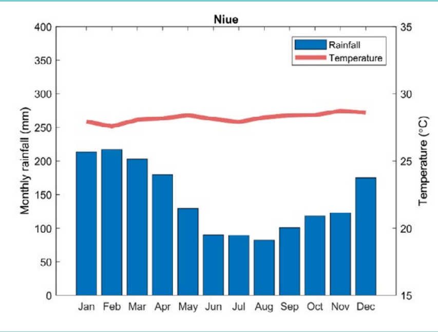
Figure 1.2. Mean annual cycle of rainfall and temperature in Niue in 1981-2010 (rainfall uses ERA5, temperature uses HadCRUT5, see Methods in Section 8).
