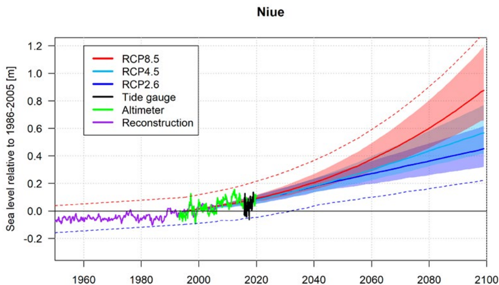
Figure 5.2 Sea level rise projections for Niue. The tide gauge record of relative sea level in Niue is indicated in black, the satellite record in green and reconstructed sea level data is shown in purple, all are monthly means without seasonal cycles and referenced to mean sea level between 1986-2005. Multi-model-mean projections from 1995–2100 are given for the RCP8.5 (red solid line), RCP4.5 (cyan solid line) and RCP2.6 emissions scenarios (blue solid line), with the 5–95% uncertainty range for RCP8.5 and RCP2.6 shown by the red and blue shaded regions respectively. The dashed lines are an estimate of interannual variability in sea level (5–95% uncertainty range) and indicate that individual monthly averages of sea level can be above or below longer-term averages.
