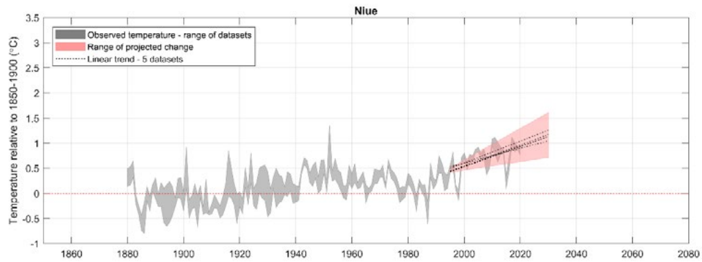
Figure 2.4 Average annual temperature of the Niue region relative to 1850-1900 (°C; grey band indicates range of five global temperature datasets), the reported range of projected change from PACCSAP is shown as a red wedge (the starting point allows for the difference between the five datasets) and the linear trend of smoothed observations for 1995-2020 plotted and extrapolated forward to 2030 (one dotted line for each dataset).
