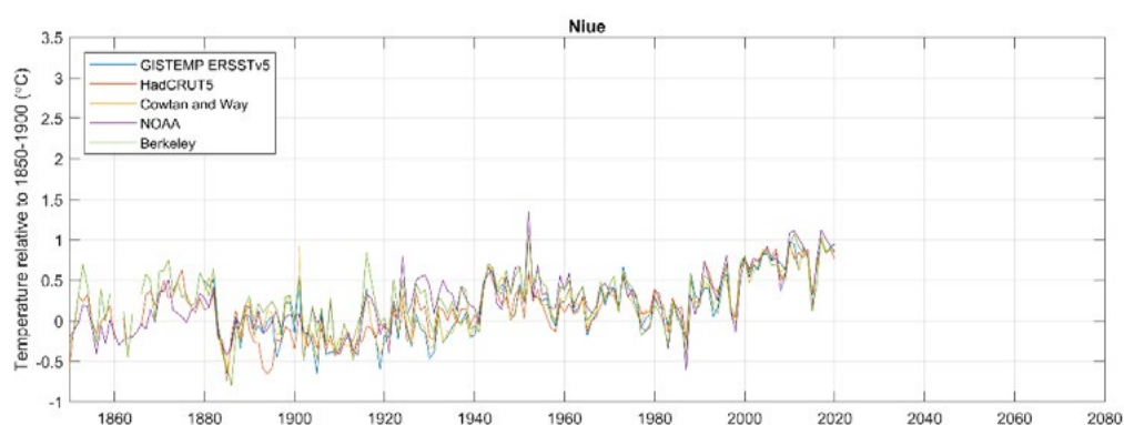
Figure 2.1. Average annual temperature of the Niue region relative to 1850-1900 in five global datasets (see Methods, Section 8 for details).
