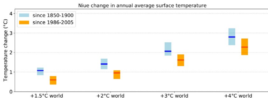
Figure 4.5. Change in the average annual temperature of the Niue region at different global warming levels, from the 1850-1900 baseline, and from the more recent baseline of 1986-2005. The bars represent multi-model median and 10th-90th percentile range.
