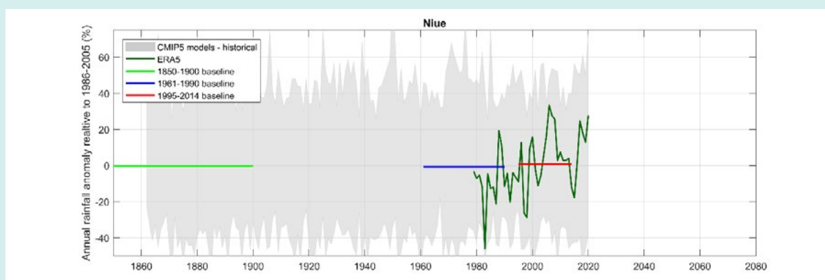
Figure 3.1 Area-average of Niue annual rainfall (%) relative to the 1986-2005 period from gridded observations (ERA5 shown, results are similar from GPCP, CMAP and ERA5), the range of CMIP5 models (grey band). Coloured horizontal bars show the average of all models for the baseline periods described in the legend.
