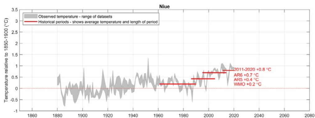
Figure 2.2 Average annual temperature of Niue relative to 1850-1900 (°C; grey band indicates the range of five global temperature datasets) and the climate average for four different historical periods (baselines), as marked:
