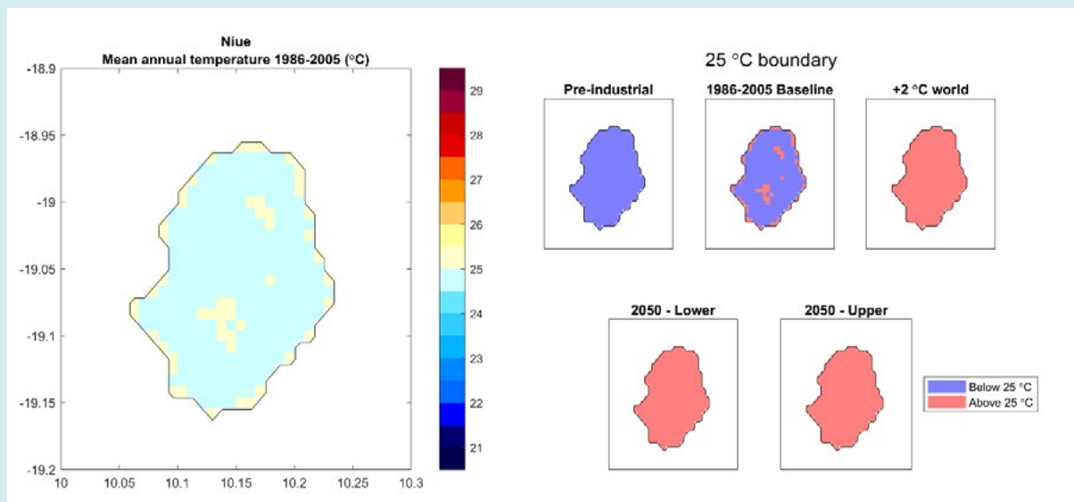
Figure 7.1. The average annual temperature in 1986-2005 in Niue (left: the 'WorldClim' high-resolution climate surface adjusted for the baseline used), and the area of the island above or below the 25°C boundary for various scenarios (right).
