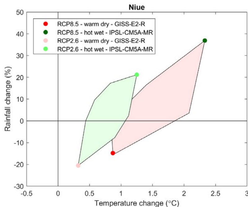
Figure 6.1 Modelled change in annual temperature and rainfall in the Niue region between 1986-2005 and 2040-2059 from CMIP5 models (coloured shapes), showing the selected models that are representative of a warm dry future and a hot wet future for RCP2.6 (low case: green polygon) and RCP8.5 (high case: red polygon).
