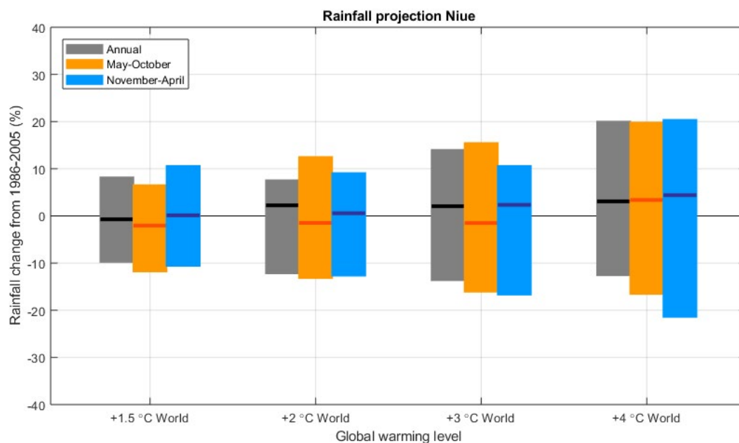
Figure 4.6. Change in the average annual and 6-month seasonal rainfall in the Niue region at different global warming levels relative to the 1986-2005 baseline. The bars represent multi-model median and 10th-90th percentile range.
