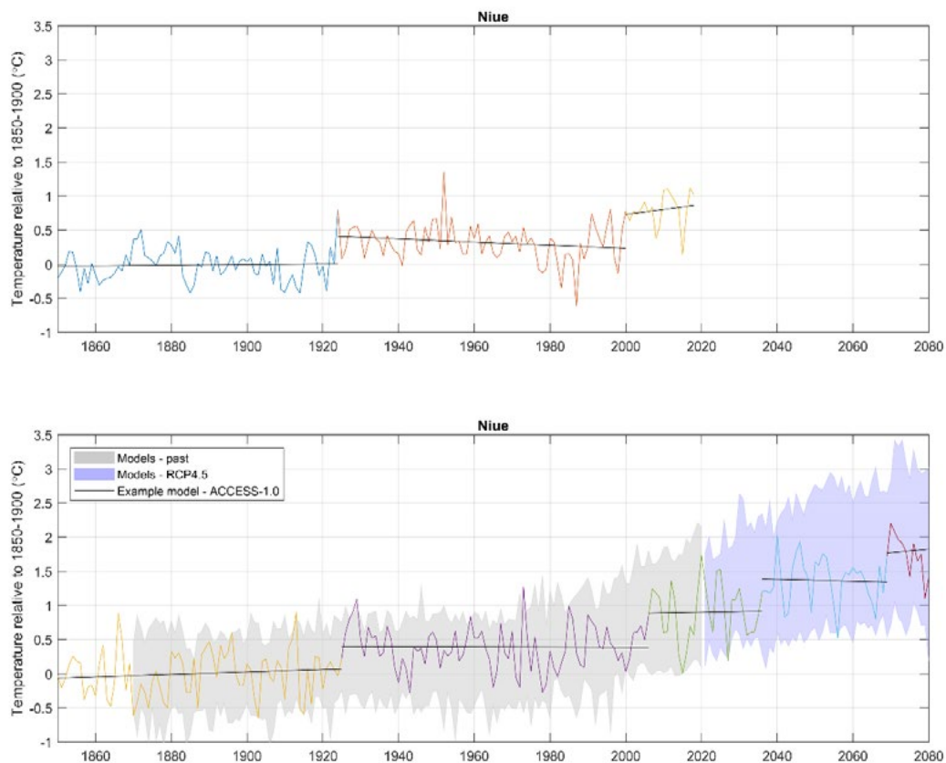
Figure 2.7. Annual average temperature relative to the 1850-1900 (°C) baseline showing detected eras separated by breakpoints (see Data and Methods): top: in observations (Cowtan and Way 2014) showing three eras, early in the time series (blue), then ‘jump’ to a warmer period through mid to late 20th Century (orange), and the warmer 2000s (yellow); and bottom: an example model simulation, showing step-like changes throughout the past and future. Example model simulation is from ACCESS-1.0 under moderate emissions RCP4.5 (results are similar but with lower background warming in RCP2.6, and higher background warming in RCP8.5).
