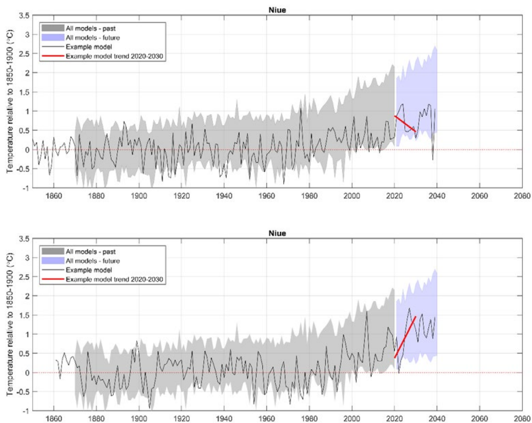
Figure 2.5. Average annual temperature in Niue relative to 1850-1900 (°C) simulated in CMIP5 models, showing the range of all models (historic; grey band, future; blue band) and example model simulations (black line) with the linear trend for 2020-2030 marked (red line); top: an example with suppressed warming in 2020-2030 due to climate variability, bottom: an example where variability enhances the warming trend in 2020-2030.
