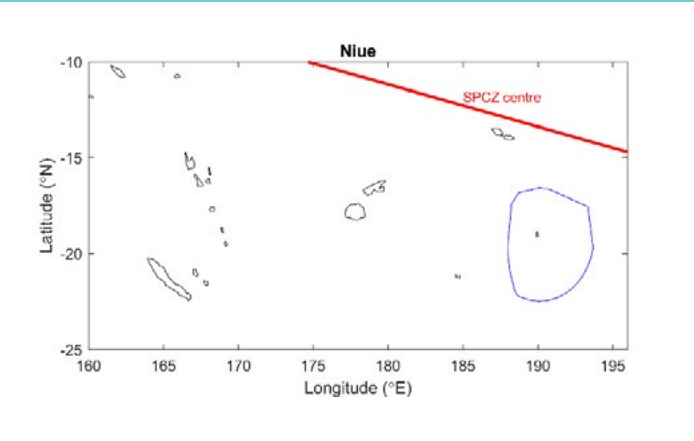
Figure 1.1. Map of Niue (top) and the mask area (bottom) for calculating areal averages from gridded observational data and climate models' outputs.
