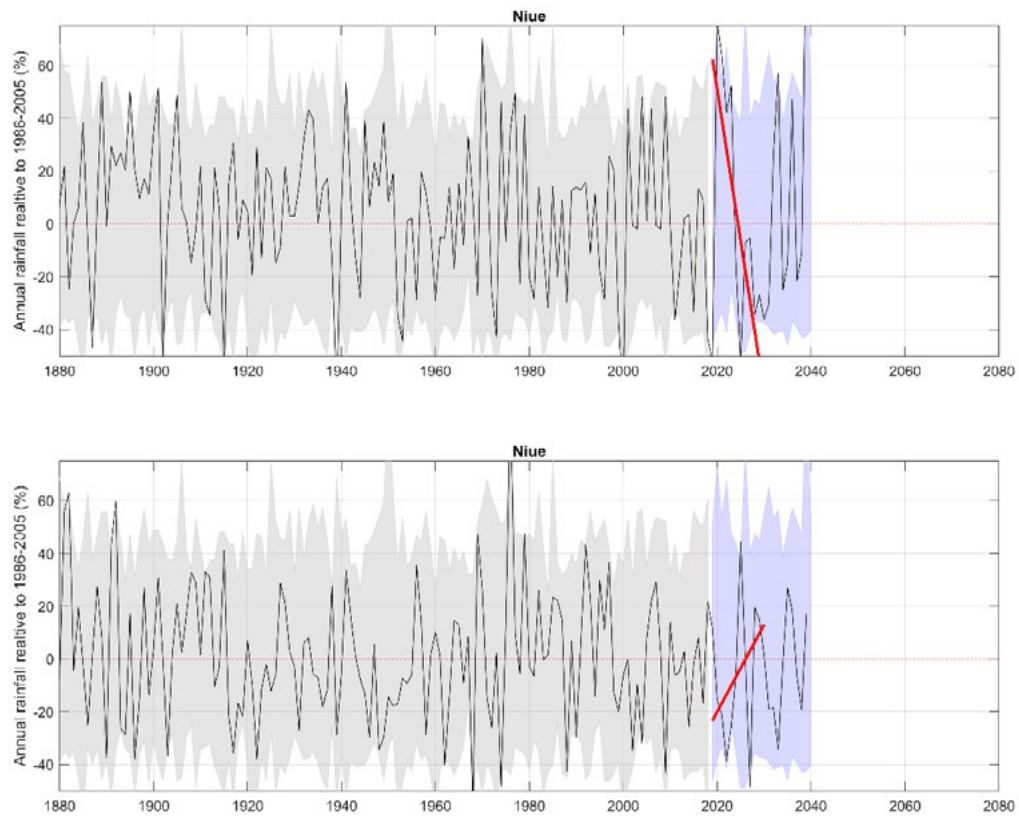
Figure 3.2 Mean annual rainfall of the Niue region relative to 1986-2005 (%) from the group of CMIP5 models (grey band: historic, blue band: future), with an example model run shown in each panel (black line) highlighting the different possible trend in 2021-2030: (top) a model showing a decrease (red trend line in the top panel), and (bottom) a model showing an increase (red trend line in the bottom panel).
