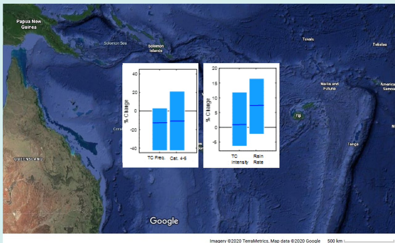
Figure 5.1 Southwest Pacific TC activity projection for a 2°C global warming. The bars on the left indicate a likely decrease in the total number of TCs, and a likely decrease but possible increase in severe (category 4-5) TCs. Bars on the right plot indicate a likely increase (but possible decrease) in the average intensity of TCs, and the very likely increase in the rainfall they bring. Shown are the median (blue line) and the 10th–90th-percentile ranges (blue bars). (Information used to construct this figure is derived from Knutson et al. 2020).
