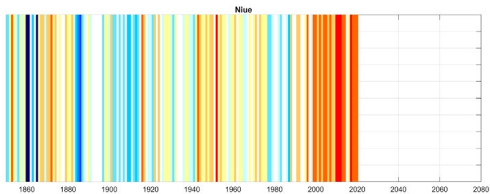
Figure 2.3 Niue temperature relative to 1961-1990 through time presented as ‘climate stripes’ devised by Hawkins (2018): red = hotter, blue = cooler (using the Berkeley dataset).
