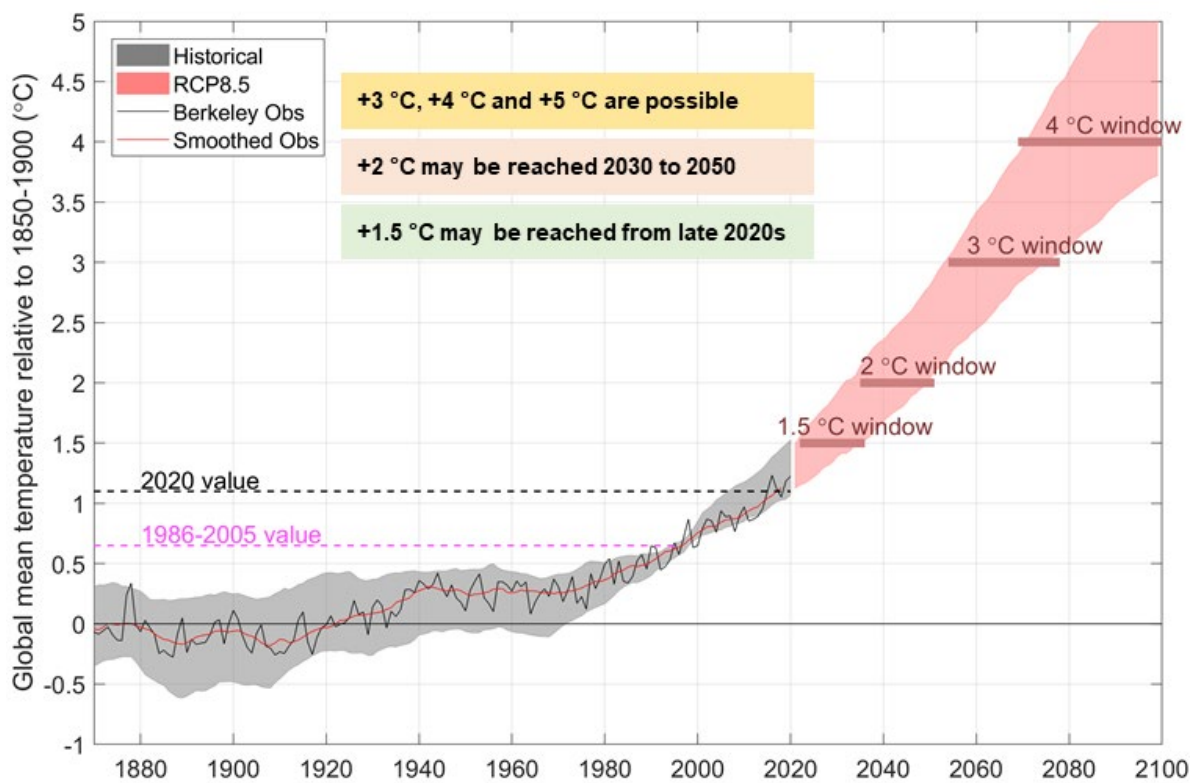
Figure 4.2 As for Figure 4.1 but showing a future under the very high emissions pathway (RCP8.5)
